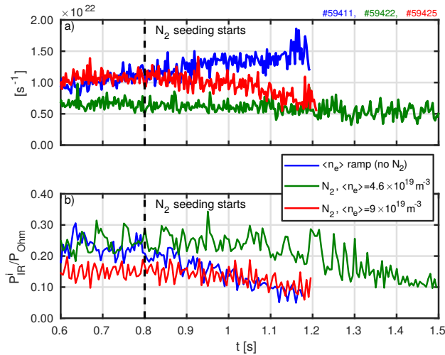
Figure 5. (top) Evolution of the integrated inner target ion flux as a function of time for the three different cases discussed in this paper. The vertical dashed line indicates the start of the N 2 -seeding for the two cases where N 2 is injected. (bottom) Integrated power flux towards the inner target as measured by an infrared thermography system for the different cases.
