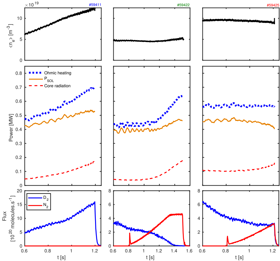
Figure 2. Time traces of the line-averaged density \langle n_e \rangle (top), the evolution of the total ohmic heating, the core radiated power P_{rad}^{core} (estimated from the bolometry reconstruction) and the power P_{SOL} going into the SOL (middle), and the evolution of the molecules fluxes ( D_2 and N_2 ) for the different scenarios studied in this paper (bottom).
