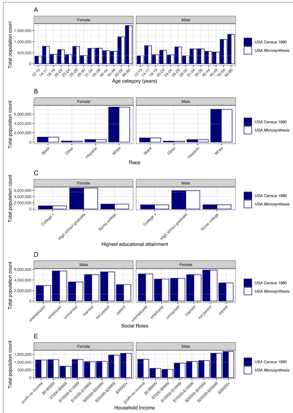
Figure 2. Validation of Micro-synthesis for the USA 1980:- modelled synthetic population compared to observed 1980 Census data for age, sex, race/ethnicity, education, social roles status and income.
