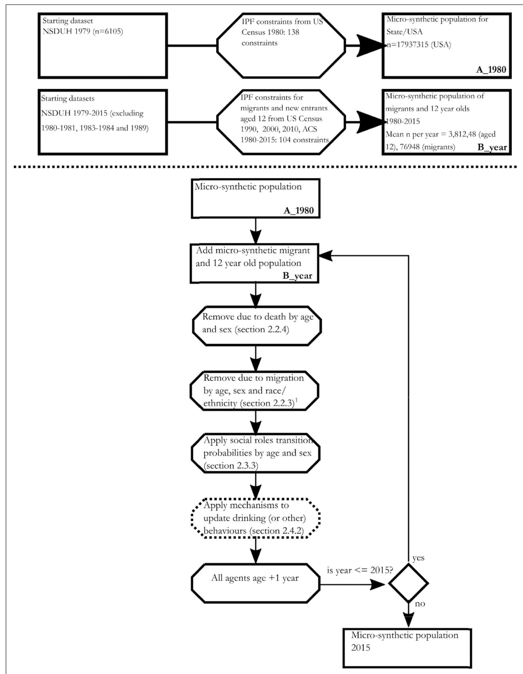
Figure 1. Schematic describing the steps taken to generate the baseline and migrant and 12-year-old populations over time, and the steps taken during each year of the microsimulation over time.
