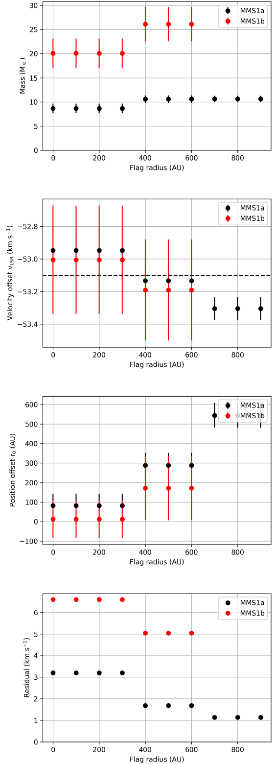
Fig. A.2. Best-fit results for the tests of flagging the inner region around the YSO. The routine was applied to the PV diagrams from the \text{H}_2\text{CO} (3_{0,3}-2_{0,2}) image. The error bars are the standard deviations from the least-squares fits. The horizontal line in the velocity plot is the systemic velocity of the source IRAS 23033+5951.
