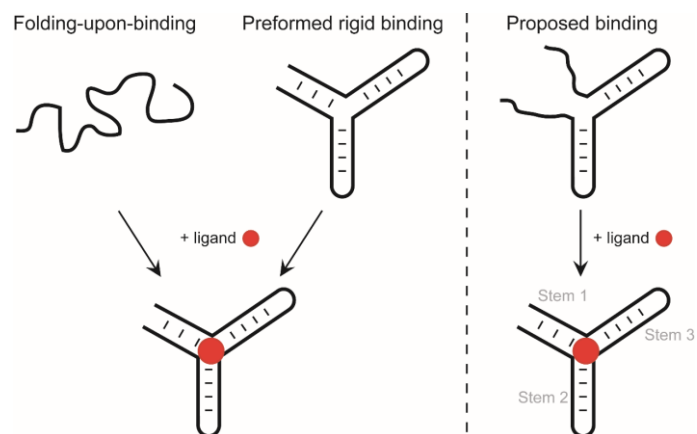
Figure 4. Schematic representation of binding modes for cocaine-binding aptamers with the ligand quinine (red circle). Binding of the ligand might occur via two extreme mechanisms: folding-upon binding of the aptamer and binding to preformed rigid aptamers. Most likely is a scenario in which stem 1 is formed upon binding (proposed binding) as suggested in the literature [53,54].
