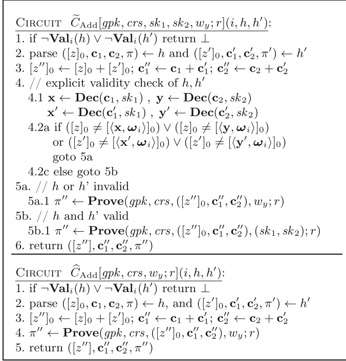
Fig. 4. Circuits for addition of group elements used in Lemma 1. \hat{pp} includes gpk = (pp_0, pk_1, pk_2, [\mathbf{W}]_0, \text{TD}, \tilde{y}) where \tilde{y} \in \text{TD} (also includes a hiding CRS \tilde{crs}' ). Both circuits also have hard-coded (the) witness w_y to \tilde{y} \in \text{TD} . Top: sk_1, sk_2 are used to produce \pi'' on valid inputs. Bottom: w_y is always used to produce \pi'' .
