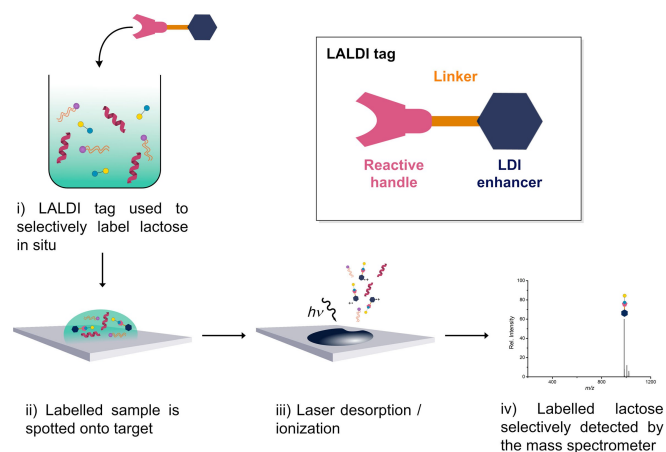
Figure 1. Concept: LALDI tags as a tool for MS-based carbohydrate detection and analysis. The figure shows the general workflow for the analysis of carbohydrates in a biological sample (in this study: lactose in cow's milk) using LALDI-MS. The inset shows the general LALDI tag design: an LDI-enhancing label (dark blue) to facilitate matrix-free laser desorption/ionisation, a linker (orange) to improve the aqueous solubility of the tag, and a reactive handle (pink) that provides a quick and reliable method to selectively label carbohydrates.
