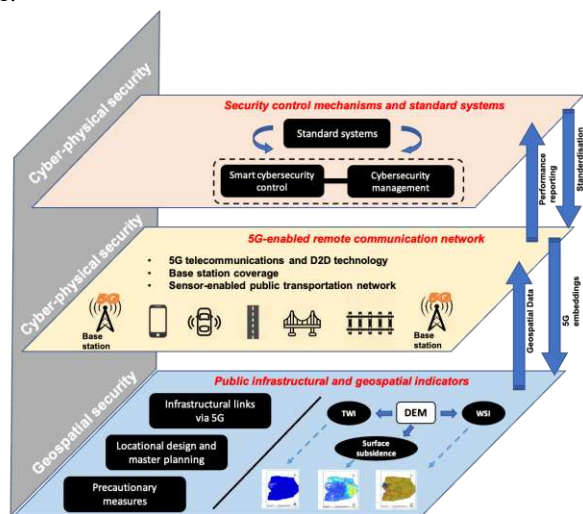
Fig. 1. The Architecture of STSS
