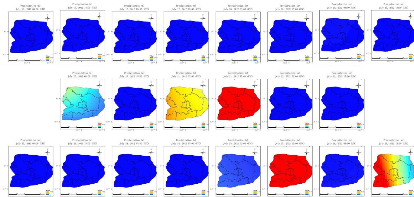
Fig. 6. Dynamic schema of precipitation in Beijing from July 16, 2012 to July 26, 2012 (two images per day at 3:00 and 15:00 UTC)
