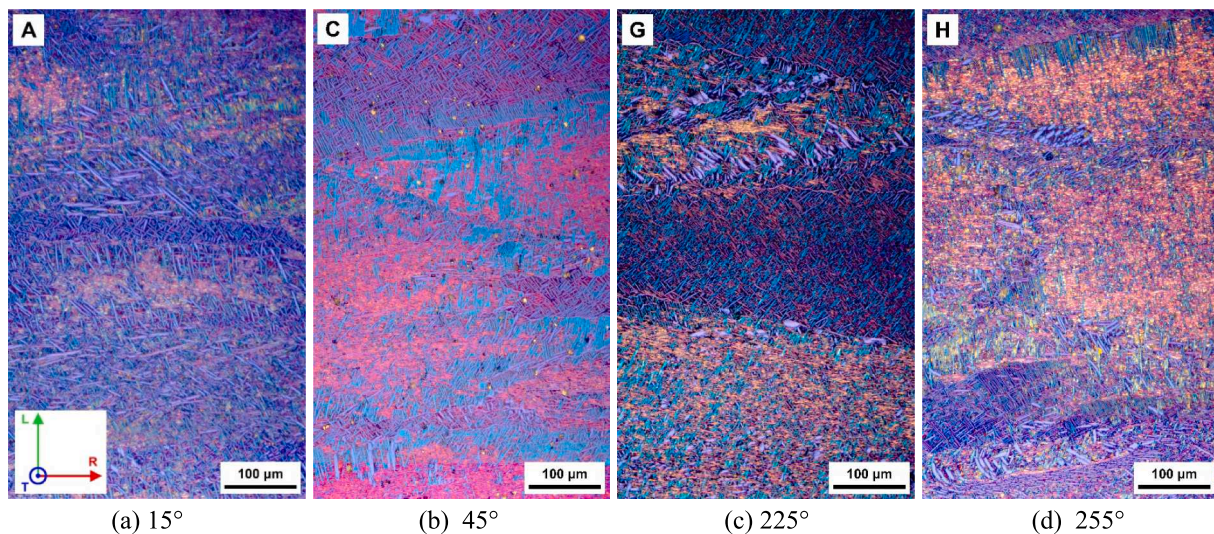
Fig. 5. Cross polarised light micrographs of Ti-6246 at different circumferential locations of the disc after chemical etching.
