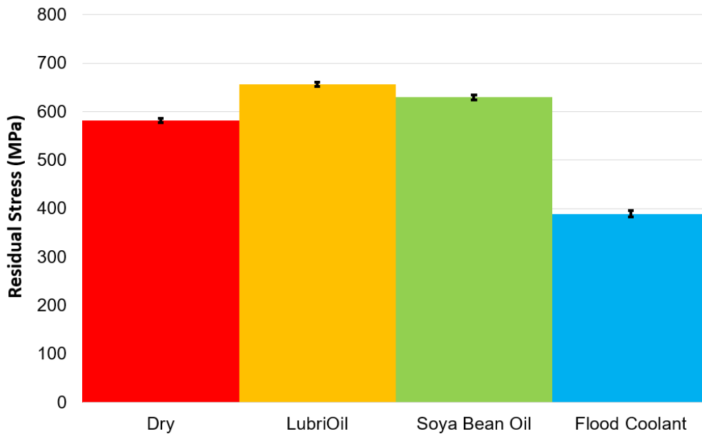
57 58 59 Figure 11 - Transverse residual stress in milling with different machining strategies. 60 61 62 63 64 65
