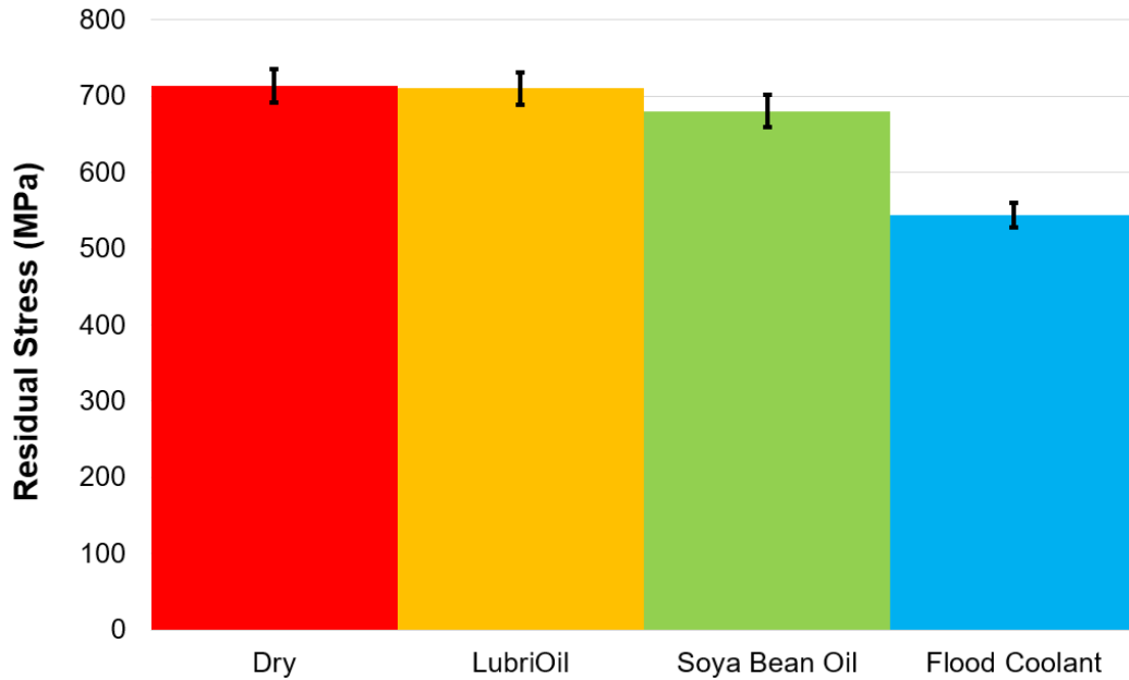
31 32 33 Figure 10 - Longitudinal residual stress in milling with different machining strategies. 34
