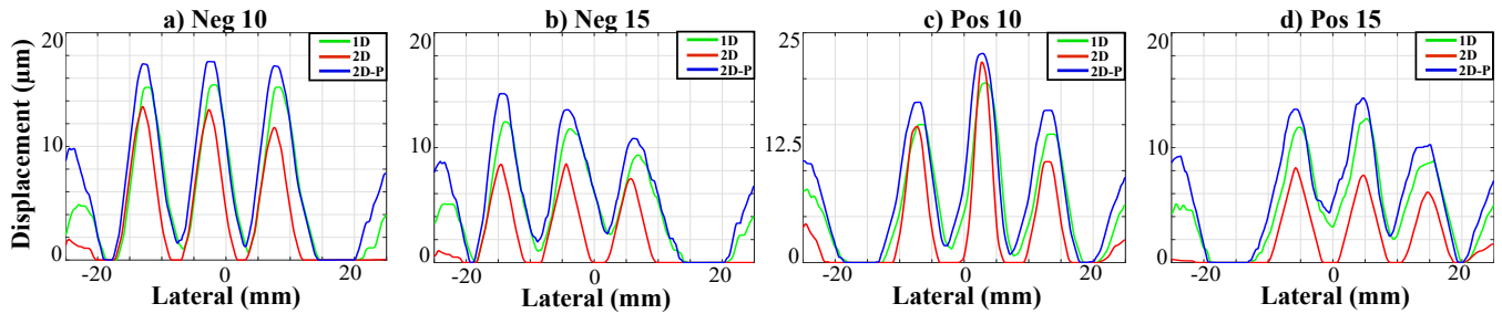
Fig. 3. Displacement amplitudes are plotted for 1D , 2D conventional and 2D proposed methods for each push beam ( -10^\circ, -15^\circ, +10^\circ, +15^\circ ) map in (a,b,c,d) plots, respectively. The displacement data is selected from a sub-frame with dimensions from 13 mm to 20 mm axially, all lateral points and then averaged along the axial direction. The proposed scheme produced an average improvement of 2.01 \mu\text{m} and 4.4 \mu\text{m} compared with the 1D axial cross-correlation and 2D cross-correction based methods, respectively.
