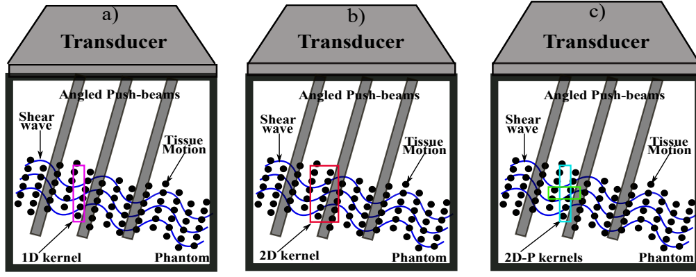
Fig. 1. The schematic diagram of displacement estimating scheme for angled shear wave with 1D axial kernel (1a), 2D kernel (1b), and 2D proposed kernels (1c). Gray bars indicate push-beam direction to generate angled shear waves, while shear waves direction is denoted by blue waves shown. In the 1D method, an axial kernel is selected, while 2D method use 2D data to produce both axial and lateral motion estimations. In the proposed 2D method, separately 1D axial and lateral tracking are used (1c) and both component values are used for calculating angled displacement vectors.
