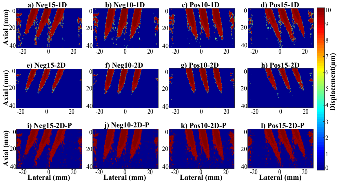
Fig. 4. Displacement maps for 1D, 2D full kernel and 2D proposed displacement estimation methods for push-beam angles as labeled on the images. The 1D axial method based images (a-d) produced inter-beam artifacts, simultaneously compromising on the lateral component of the displacement vector. Using the 2D kernel method (e-h), noise is fully suppressed at the push-beam contours but the displacement amplitude is reduced while the proposed 2D estimation method (i-l) is able to produce both axial and lateral components of displacements and improved the displacement vector amplitude effectively.
