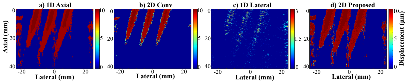
Fig. 2. The shear wave induced displacement maps are produced for -15^\circ push-beam angle using displacement estimation methods as labeled on top of the each image. Displacement maps are processed using received RF data instantly after the push-beams are stopped and tracking beams are applied. It can be observed that, the 1D axial method produced images with noisy estimates between the push-beams, while the 2D conventional method removed the artifacts by averaging neighboring values due to a larger kernel size in the lateral direction. The Proposed scheme used axial and lateral displacement components separately, and calculated 2D displacement vector. The proposed technique is able to estimate the lateral displacement component which eventually improves displacement estimation.
