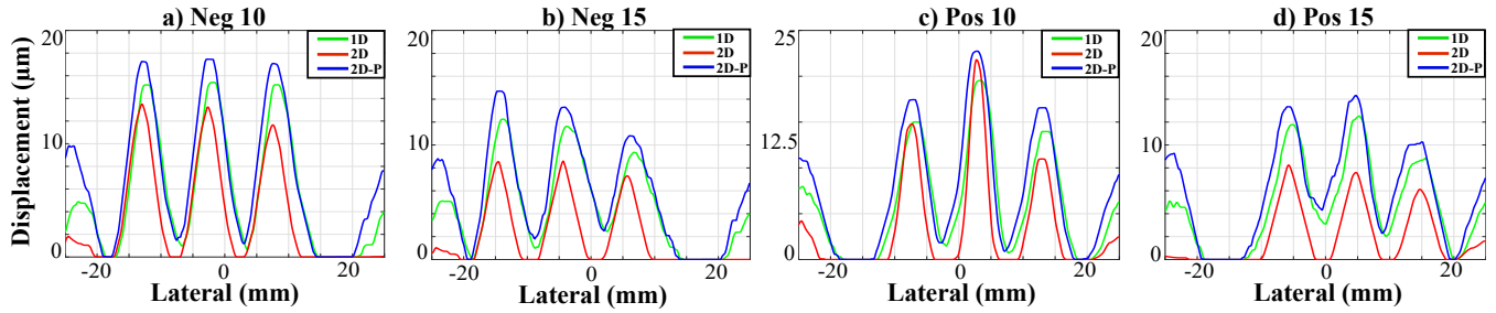
Fig. 3. Displacement amplitudes are plotted for 1D , 2D conventional and 2D proposed methods for each push beam ( -10^\circ , -15^\circ , +10^\circ , +15^\circ ) map in (a,b,c,d) plots, respectively. The displacement data is selected from a sub-frame with dimensions from 13 mm to 20 mm axially, all lateral points and then averaged along the axial direction. The proposed scheme produced an average improvement of 2.01 \mu\text{m} and 4.4 \mu\text{m} compared with the 1D axial cross-correlation and 2D cross-correction based methods, respectively.
