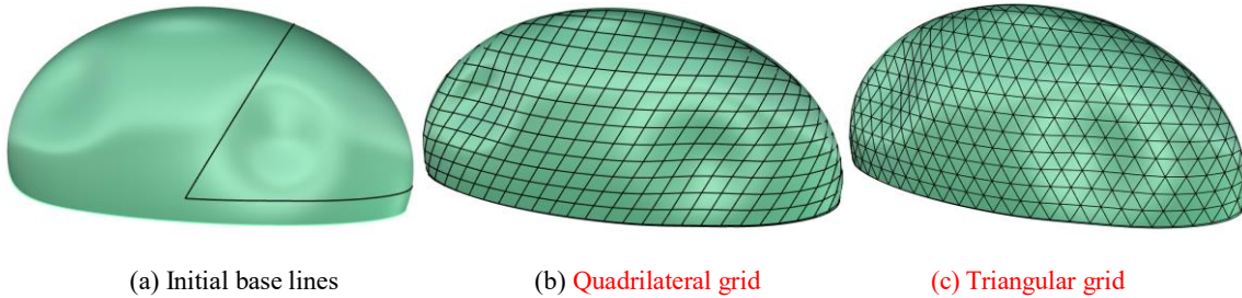
Fig. 17 The grids generated by CBPM ( R=2.1m, \alpha = 60^\circ )
