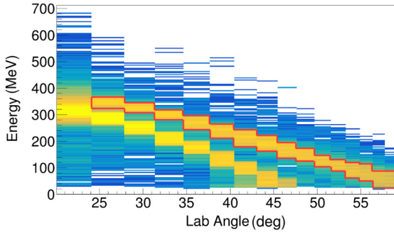
FIG. 1. The particle spectrum collected in the DSSSD detector, displaying the projectile and target kinematics for the Coulomb excitation of ^{130}\text{Xe} on a ^{94}\text{Mo} target. The red outline indicates the region gated on for target-like events.
