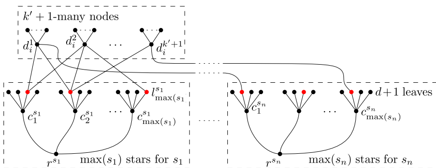
Fig. 2 Example of the gadget in Theorem 2
