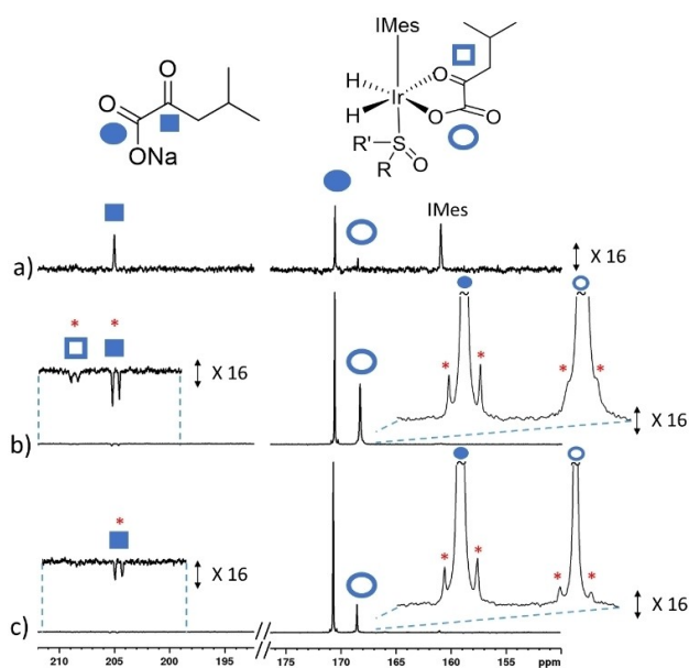
Figure 2. Partial hyperpolarized ^{13}\text{C} NMR spectra when samples containing [\text{IrCl}(\text{COD})(\text{IMes})] (5 mM) and a) KIC and b-c) KIC-1- ^{13}\text{C} are shaken with a) dimethylsulfoxide (22.5 mM), b) dimethylsulfoxide (50 mM) and c) methylphenylsulfoxide (50 mM) and p\text{-H}_2 (3 bar) in methanol- d_4 (0.6 mL) for 10 seconds in a mu-metal shield at c.a. 1 \mu\text{T} . Note the signals marked by a red asterisk denote singlet magnetization of naturally abundant KIC-1,2- ^{13}\text{C}_2 .
