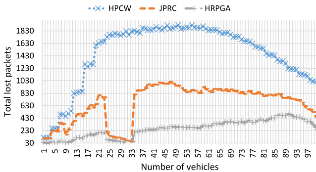
FIGURE 7 Total lost packets of 100 vehicles
