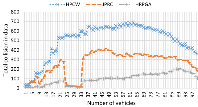
FIGURE 10 Total data collision of 100 vehicles
