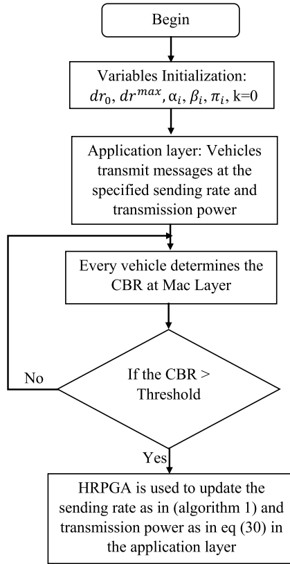
FIGURE 2 A block diagram of the HRPGA
