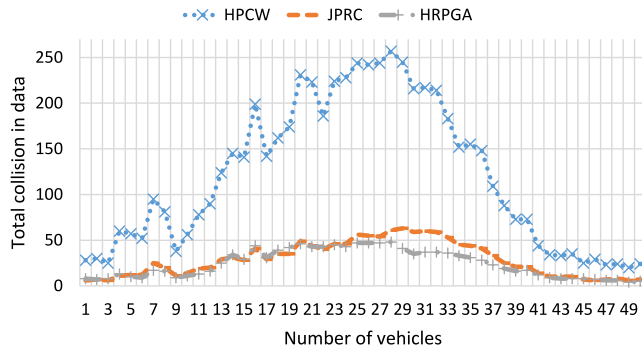
FIGURE 9 Total data collision of 50 vehicles
