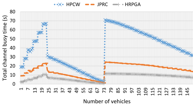
FIGURE 5 Total channel busy time of 150 vehicles
