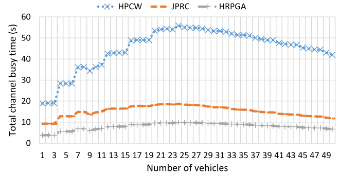
FIGURE 3 Total channel busy time of 50 vehicles
