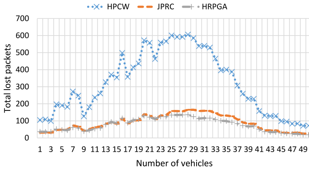
FIGURE 6 Total lost packets of 50 vehicles
