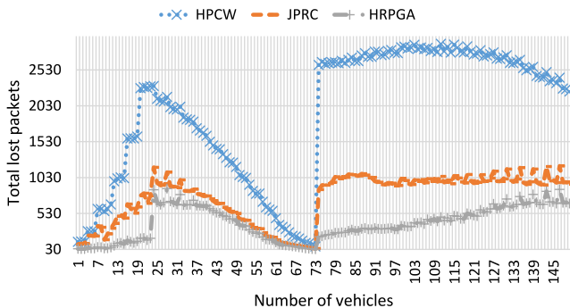
FIGURE 8 Total lost packets of 150 vehicles
