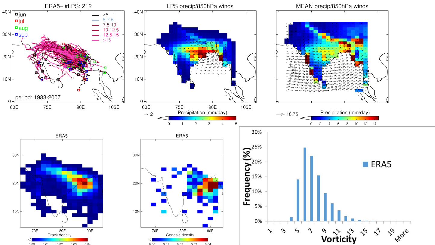
Fig. 1 Monsoon LPS diagnosed in ERA5 re-analysis for 1983-2007 with APHRODITE land precipitation statistics. On the top row: the first panel on left hand-side shows LPS trajectories with the total number of LPS in title. The coloured squares indicate the starting point and month of each track. The colour of the trajectories indicates the strength in terms of relative vorticity ( 10^{-5} s^{-1} at native resolution). The second panel from left shows LPS contribution to JJAS seasonal precipitation (mm/day) and 850 hPa winds (m/s, black vectors). The third panel from left shows Jun-Sept seasonal mean precipitation (mm/day) and 850 hPa winds (m/s, black vectors). All data is plotted on a 200km ( N96; 1.875^\circ \times 1.25^\circ ) grid. Bottom row shows TRACK DENSITY, GENESIS DENSITY and a HISTOGRAM of LPS intensity. The intensity is shown in terms of relative vorticity (in units of 10^{-5} s^{-1} ) filtered to T42 resolution (as used in tracking) at the centre of the system at the 850hPa level, and includes all 6-hourly time-steps during LPS lifetime. These ERA5 figures have been generated using Copernicus Climate Change Service Information 2020.
