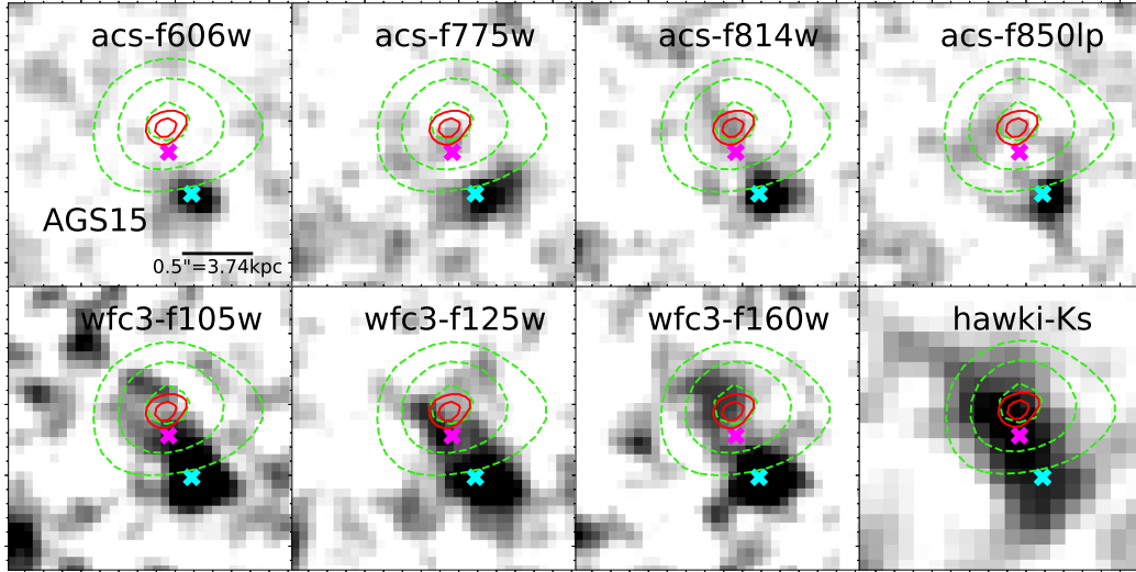
Fig. 9. Same as in Fig. 6, but for AGS15. The cyan “x” denotes the optical bright neighbor, ID_{\text{CANDELS}} = 3818 ( z_{\text{phot}} = 4.27 ). The magenta “x” denotes the detection in K_s -band by ZFOURGE, ID_{\text{ZFOURGE}} = 6755 ( z_{\text{phot}} = 3.47 ).
