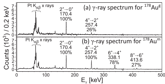
FIG. 8. Background-subtracted singles \gamma -decay spectra measured by the LEGe following the \beta^+ /EC decays of (a) ^{178}\text{Au}^g and (b) ^{178}\text{Au}^m . The relevant peaks are labeled with their energies (in keV), along with the spins and parities of the initial and final states in ^{178}\text{Pt} and their intensities corrected for \gamma -ray detection efficiency, normalized to the intensity of the 170.4-keV 2^+ \rightarrow 0^+ transition.
