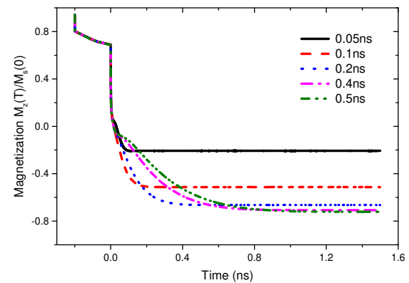
FIG. 8. (Color online) The time variation of the magnetization, after heating to T_c , for the thin film magnetization, over a range of cooling rates. For a cooling rate below 0.2ns the level of magnetization reversal is significantly reduced.
