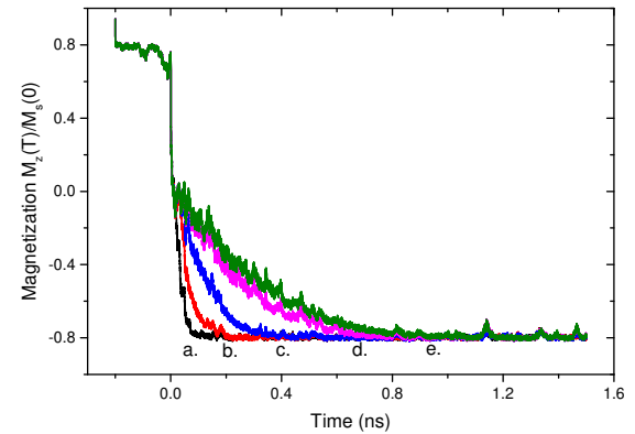
FIG. 7. (Color online) The linear reversal case (heating to T_c ), for a single grain, over a range of cooling rates. The reversal of the individual grain's magnetization is seen to happen at a greater rate with the quicker cooling time. The cooling times are as follows: a. 0.05ns, b. 0.1ns, c. 0.2ns, d. 0.4ns, e. 0.5ns.
