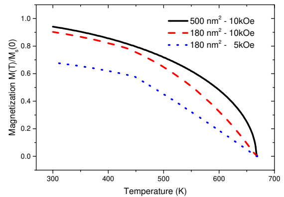
FIG. 9. (Color online) Field cooled magnetisation curves as a function of particle sizes 180 \text{ nm}^2 ( 900 \text{ nm}^3 ) and 500 \text{ nm}^2 ( 2500 \text{ nm}^3 ) and magnetic field. The cooling rate is 500 \text{ K ns}^{-1} . The system becomes increasingly blocked as the size of both particle and applied field are reduced.
