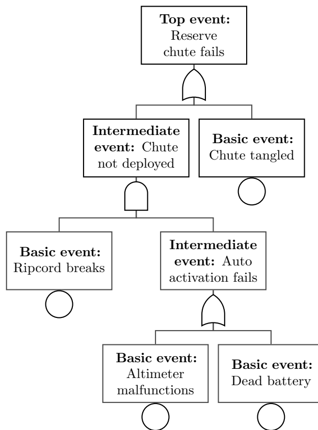
Figure 2: An example fault tree for a reserve parachute system [11].
