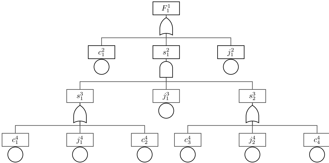
Figure 6: A fault tree of a failure mode F_1 where the superscript denotes the hierarchy level and the subscript is an identifier.
