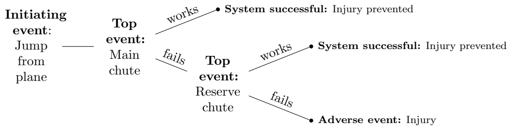
Figure 1: An example event tree for a parachute system to prevent fall injuries [11].
