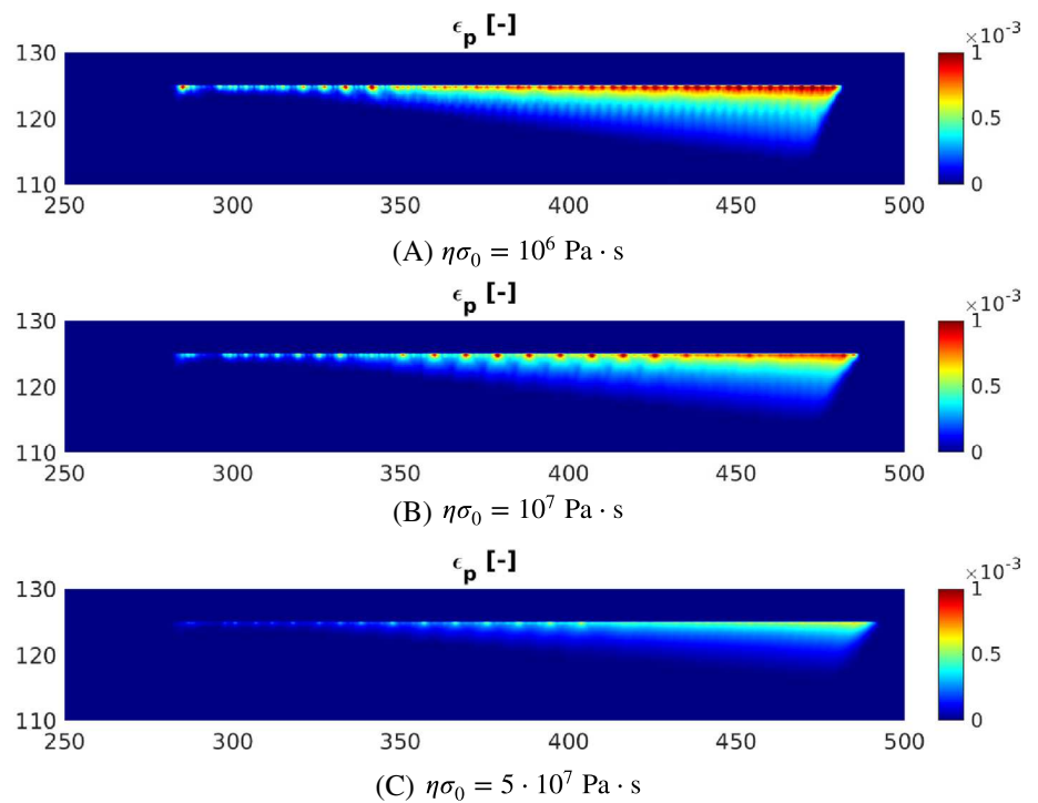
FIGURE 16 Plastic strain after t = 1.2 s around the right fracture tip using a standard continuum with the 320 \times 50 mesh. (A) \eta\sigma_0 = 10^6 Pa \cdot s; (B) \eta\sigma_0 = 10^7 Pa \cdot s; (C) \eta\sigma_0 = 5 \cdot 10^7 Pa \cdot s [Color figure can be viewed at wileyonlinelibrary.com ]
