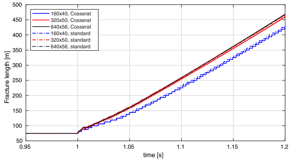
FIGURE 15 Fracture length using the 160 \times 40 , 320 \times 50 , and 640 \times 56 meshes using the standard and Cosserat continua [Color figure can be viewed at wileyonlinelibrary.com ]
