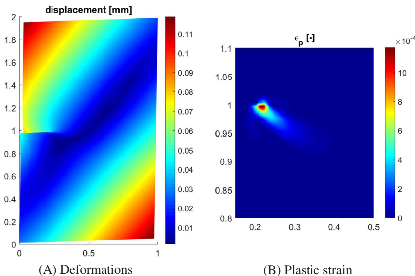
FIGURE 3 Deformations and plastic strain at t = 1.02 s for t_t = 0.4 MPa [Color figure can be viewed at wileyonlinelibrary.com ]
