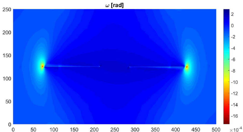
FIGURE 9 Cosserat rotation at t = 1.15 s [Color figure can be viewed at wileyonlinelibrary.com]
