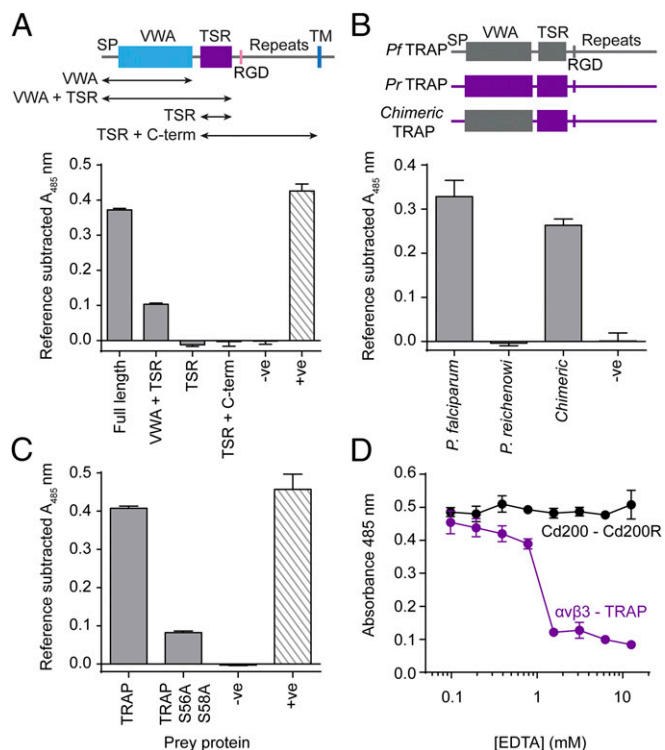
Fig. 4. The P. falciparum TRAP VWA domain is required for integrin \alpha\text{v}\beta 3 binding. (A, Upper) A series of truncations of the P. falciparum TRAP extracellular domain were expressed as pentameric preys. C-Term, C terminus; SP, signal peptide; TM, transmembrane. (Lower) Binding with integrin \alpha\text{v}\beta 3 quantified by AVEXIS. The VWA domain alone was expressed at insufficient levels for use in the assay. Only the full-length extracellular domain of TRAP was able to fully interact with \alpha\text{v}\beta 3 bait in AVEXIS; however, residual binding signal was observed for the VWA + TSR construct. (B, Upper) Replacing the VWA domain in the nonbinding P. reichenowi TRAP with the orthologous domain from P. falciparum was sufficient to confer the ability to bind integrin \alpha\text{v}\beta 3 . The entire extracellular regions of P. falciparum (Pf) and P. reichenowi (Pr) TRAP, as well as a VWA-domain replacement chimera were expressed as prey proteins. (Lower) Binding activity to integrin \alpha\text{v}\beta 3 quantified by AVEXIS. (C) Mutating two conserved serine residues within the MIDAS sequence of the P. falciparum TRAP VWA domain significantly decreased binding to \alpha\text{v}\beta 3 . TRAP and the S56A S58A TRAP were expressed as preys and used in the AVEXIS assay to test binding against \alpha\text{v}\beta 3 bait. In (A–C), the positive control (+ve) is the Cd200–Cd200R interaction and the negative control (–ve) was Cd200 bait and TRAP prey. Bars represent means \pm SD, n = 3 . A representative experiment of at least two independent experiments is shown. (D) The TRAP– \alpha\text{v}\beta 3 interaction is divalent cation dependent. Dose-dependent inhibition of the TRAP– \alpha\text{v}\beta 3 interaction, but not the Cd200–Cd200R interaction, was observed using the AVEXIS assay when prey proteins were preincubated with increasing concentrations of divalent cation chelator EDTA. Data points represent mean \pm SD, n = 3 . A representative experiment of at least three independent experiments is shown.
