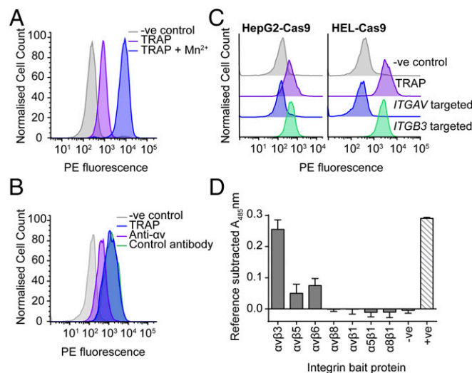
Fig. 5. The integrin \alpha\text{v} -subunit is essential for TRAP binding to HepG2 cells. (A) Binding of an oligomerized TRAP binding probe to HepG2 cells is enhanced by addition of 2 mM \text{MnCl}_2 to the buffer. (B) Binding of TRAP to HepG2 cells can be partially blocked by preincubation with an anti- \alpha\text{v} antibody (mouse IgG1 clone 272-17E6), but not an isotype-matched monoclonal antibody to another surface protein (anti-BSG mouse IgG1 clone MEM-M6/6). (C) Binding of TRAP is completely abolished in HepG2 and HEL cells in which ITGAV , but not ITGB3 , genes have been targeted using CRISPR/Cas9 technology. Negative (–ve) controls in A–C are Cd200 oligomerized around streptavidin–phycoerythrin, which does not stain cell surfaces. (D) TRAP is able to bind integrins \alpha\text{v}\beta 5 and \alpha\text{v}\beta 6 , in addition to \alpha\text{v}\beta 3 . Seven RGD-binding integrins were expressed as biotinylated bait proteins and screened by AVEXIS for interaction against TRAP prey. Positive control (+ve) is the Cd200–Cd200R interaction and the negative control (–ve) was Cd200 bait and TRAP prey. Bars represent mean \pm SD, n = 3 . A representative experiment of at least three independent experiments is shown.
