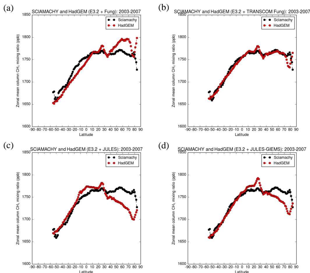
Figure 9. Comparisons of the latitudinal distribution of the average atmospheric column methane mixing ratio between the years 2003 and 2007, as derived from monthly regrided SCIAMACHY data and from the HadGEM2 runs using the FUNG (a), TRANSCOM-FUNG (b), JULES (c) and JULES-GIEMS (d) wetland emission inventories and the EDGAR v3.2 (E3.2) anthropogenic methane emission time series, sampled at co-located space and time points. Note that the SCIAMACHY data between 60 and 90° S have been removed because of their sparsity and quality.
