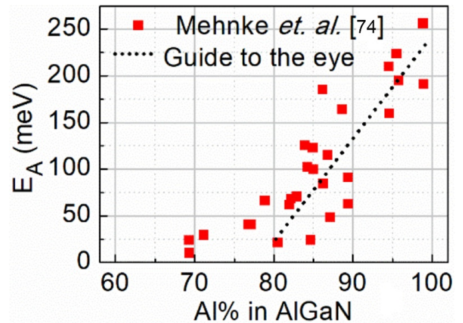
Figure 11. Donor E_A of Si in Al-rich AlGaN epitaxial films [74]. Si donor E_A in n-GaN is \sim 15 \text{ meV} , which increases to \sim 50 \text{ meV} in n\text{-Al}_x\text{Ga}_{1-x}\text{N} ( x < 0.8 ) epitaxial films [73]. Thus, nearly full ionization of free carriers at room temperature is typically observed in n\text{-Al}_x\text{Ga}_{1-x}\text{N} ( x < 0.8 ) epitaxial films.
