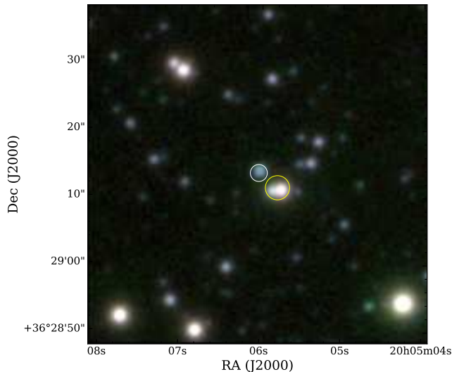
Figure 2. False color composite image centered on Gaia 18dvy (white circle) using Pan-STARRS i, z, y images. The nearby sources whose contribution was subtracted from the WISE photometry are marked by the yellow circle.
