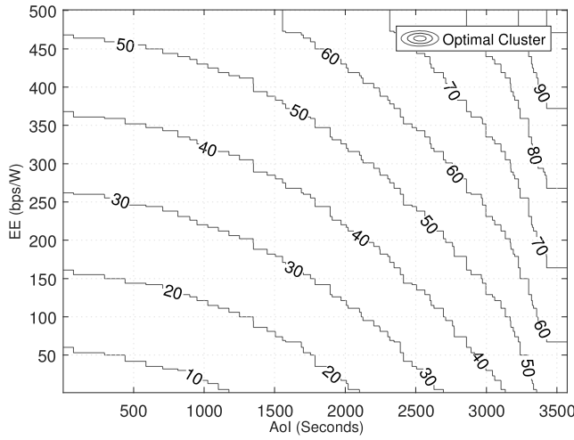
Fig. 7: Optimal Clusters for 1000x1000 m^2 area
