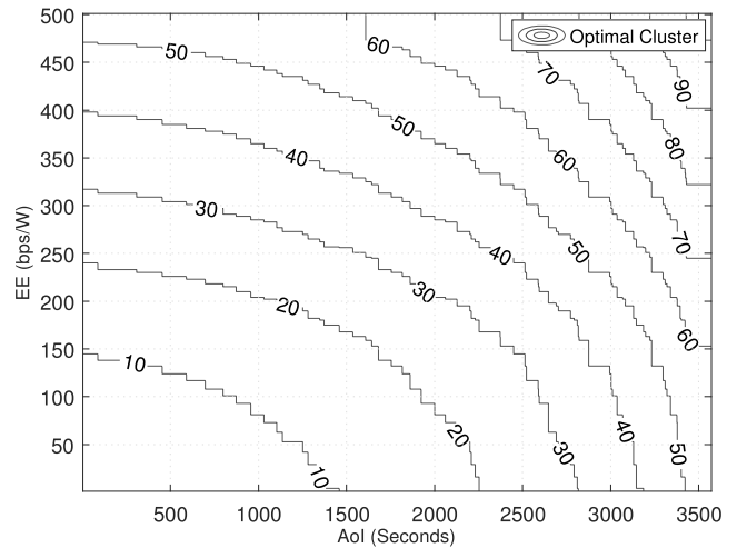
Fig. 6: Optimal Clusters for 500x500 m^2 area
