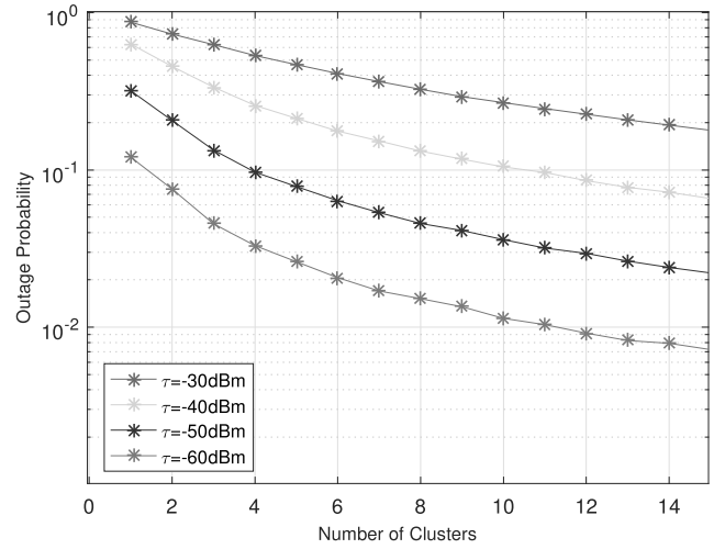
Fig. 2: Outage probability for different number of clusters
