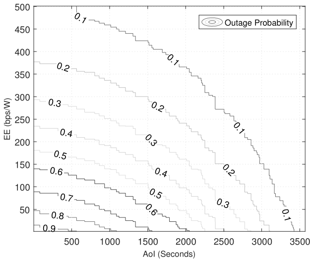
Fig. 8: Outage probability for 1000x1000 m^2 area
