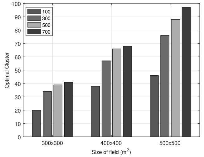
Fig. 5: Optimal Clusters for min EE=200 bps/W, max AoI=900 seconds and outage probability < \gamma
