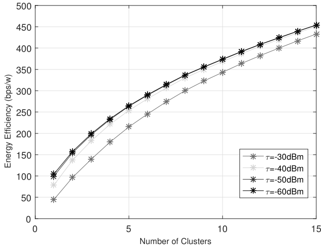
Fig. 3: EE for different number of clusters
