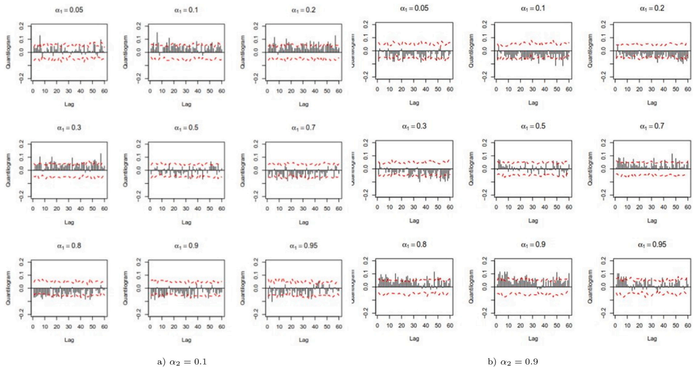
Fig. 8. Cross-quantilogram representing directional predictability from Ripple returns to Bitcoin returns. Source: To detect directional predictability from Ripple returns to Bitcoin returns, the sample cross quantilogram \hat{p}_\alpha(k) for \alpha_2 = 0.1 and \hat{p}_\alpha(k) for \alpha_2 = 0.9 . The bar graphs explain sample cross quantilograms, and the lines are the 95% bootstrap confidence intervals.
