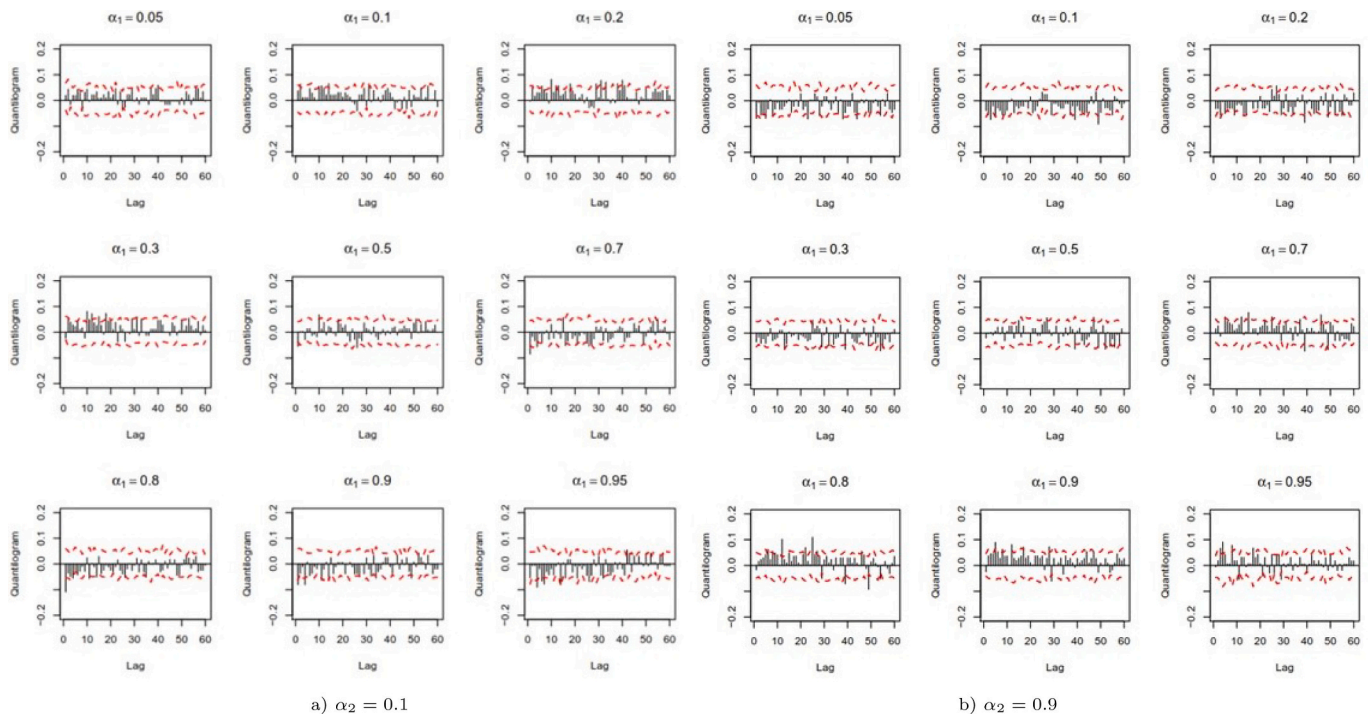
Fig. 14. Cross-quantilogram representing directional predictability from NEM returns to Bitcoin returns. Source: To detect directional predictability from NEM returns to Bitcoin returns, the sample cross quantilogram \hat{p}_\alpha(k) for \alpha_2 = 0.1 and \hat{p}_\alpha(k) for \alpha_2 = 0.9 . The bar graphs explain sample cross quantilograms, and the lines are the 95% bootstrap confidence intervals.
