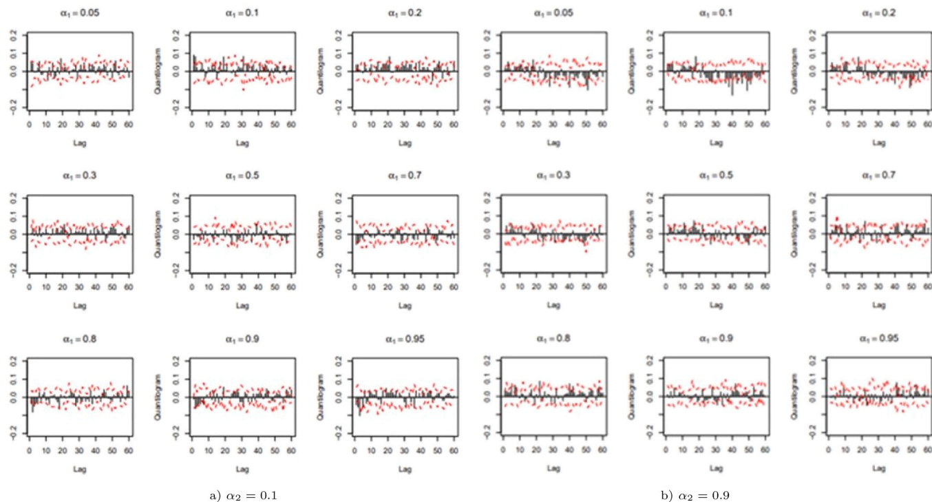
Fig. 2. Cross-quantilogram representing directional predictability from Bitcoin returns to Ether returns. Source: To detect directional predictability from Bitcoin returns to Ether returns, the sample cross quantilogram \hat{p}_\alpha(k) for \alpha_2 = 0.1 and \hat{p}_\alpha(k) for \alpha_2 = 0.9 . The bar graphs explain sample cross quantilograms, and the lines are the 95% bootstrap confidence intervals.
