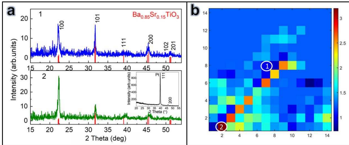
Figure 2 (a): X-ray diffraction patterns obtained from Regions 1 and 2 illustrated in Fig. 1(a). The vertical red tick marks correspond to the \text{Ba}_{0.85}\text{Sr}_{0.15}\text{TiO}_3 (PDF card 01-082-8710) indicating a match with this perovskite phase. The inset figure on the bottom right shows an X-ray diffraction pattern obtained from the SSTOP substrate, which shows the 111 and 200 reflections of Pt at 39.8 and 46 degrees, respectively. (b): Map of the 100/101 intensity ratio across the film.
