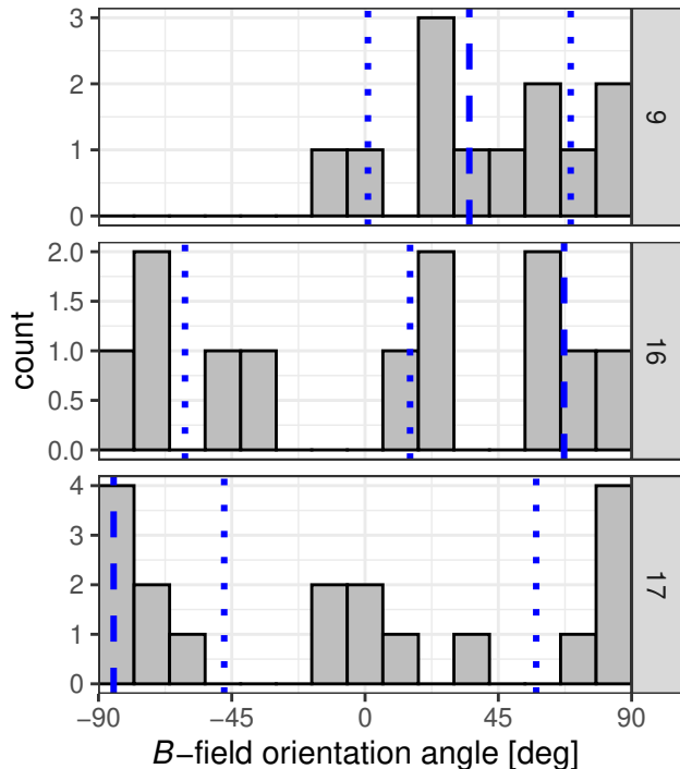
Figure 8. Same as Figure 7 but for the features that show relatively scattered B -field position angles (the circular standard deviation of the position angles > 30^\circ ).
