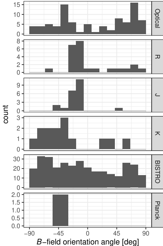
Figure 10. Histograms of the position angles for the B -field orientations observed by optical and near-infrared polarimetry. Optical data (762.5 nm) are from Goodman et al. (1990) . R -band and J -band data are from Alves et al. (2011) . K -band data are from Tamura et al. (1988) . Submillimeter data taken by BISTRO and Planck, rotated by 90^\circ , are shown for comparison. Note that the spatial coverages are different for individual observations, especially R -band and J -band data by Alves et al. (2011) , which cover only a small area south of the IRAS 4A and IRAS 4B (see text).
