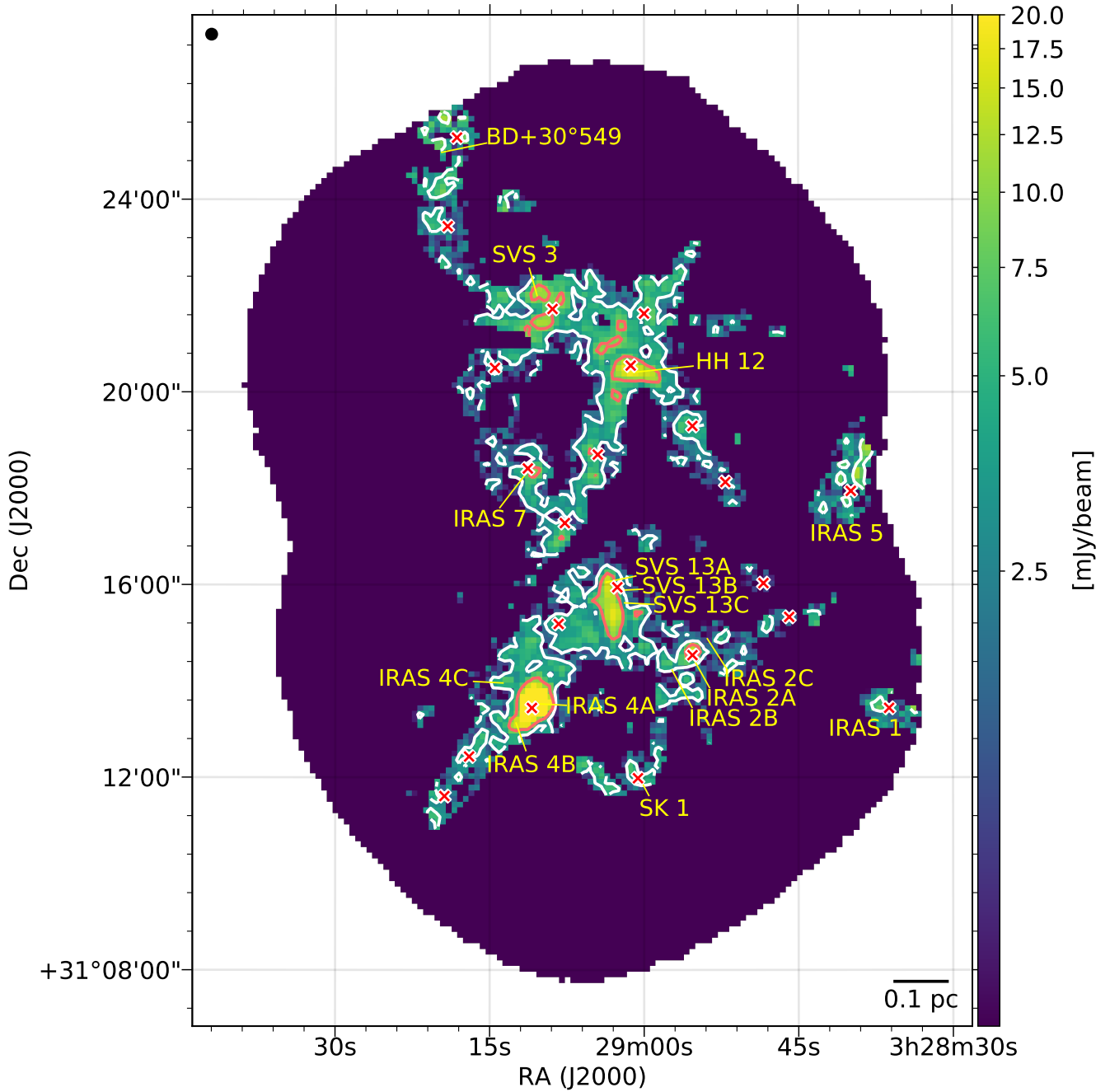
Figure 2. Polarized intensity observed at 850 \mu\text{m} . The JCMT beam ( 14''.1 ) is shown in the upper left corner of the figure. Color scale is polarized intensity, PI . Contours are for PI/\delta PI = 3 (white contour) and PI/\delta PI = 10 (orange contour). Red crosses are the same as those in Figure 1.
