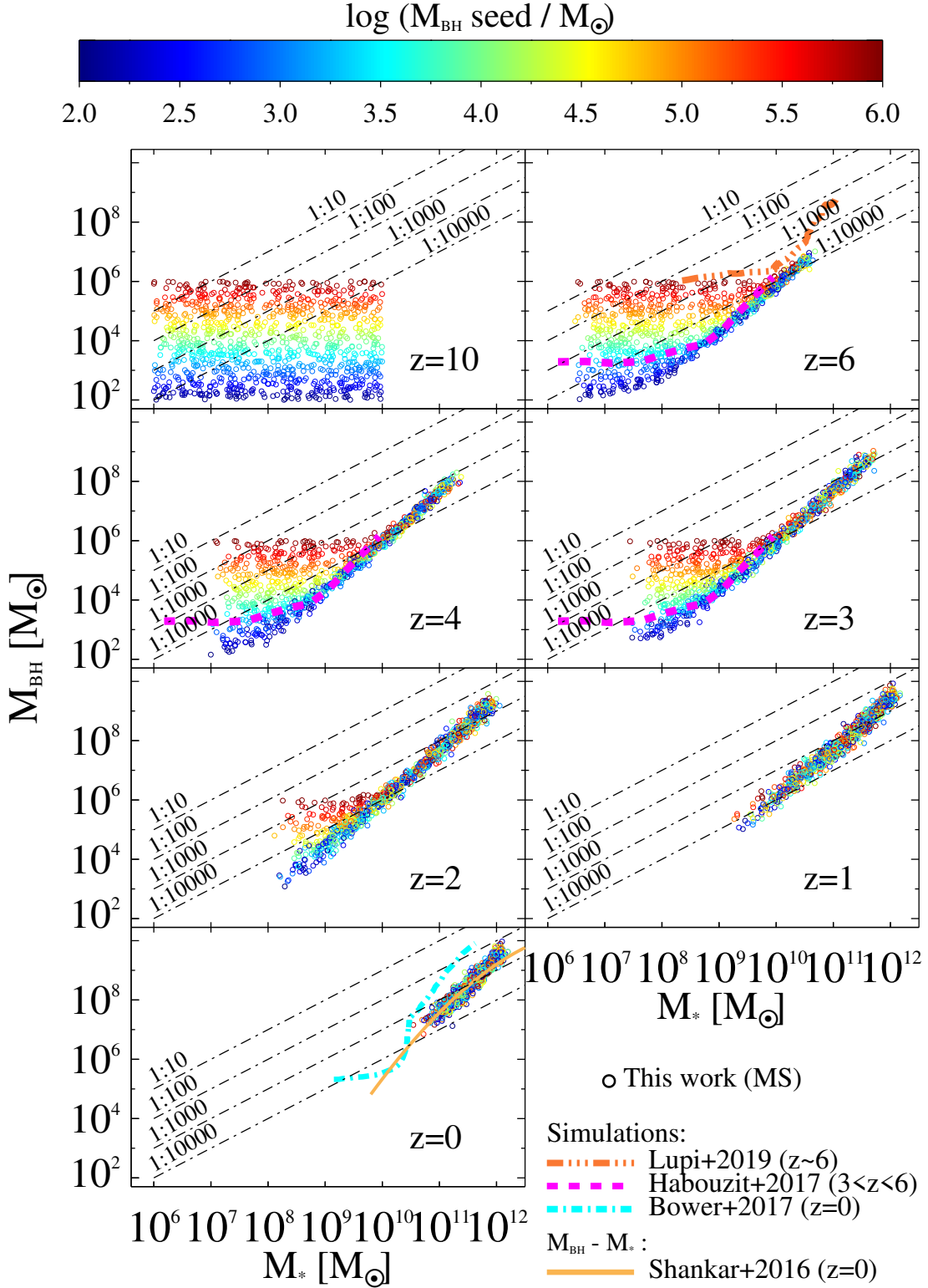
Figure 2. Cosmic build-up of SMBH and galaxy mass implied by our M_* -dependent BHAR/SFR trend (open circles). We assume uniform M_{\text{BH}} and M_* seed distributions at z_f=10 , spanning the ranges 10^2 < M_{\text{BH}} < 10^6 and 10^6 < M_* < 10^{10} M_{\odot} , respectively (top-left panel). The colorbar indicates the seed M_{\text{BH}} distribution at z_f . Dot-dashed lines mark various M_{\text{BH}}/M_* ratios. We track the evolution of M_* and M_{\text{BH}} for MS galaxies (circles), incorporating the scatter of the MS relation and the uncertainties on the assumed BHAR/SFR trend. For comparison, we show predictions of a SB galaxy at z \sim 6 (Lupi et al. 2019, orange dot-dashed line), and of normal star-forming galaxies (Habouzit et al. 2017, magenta dotted line at 3 < z < 6 ; Bower et al. 2017, cyan dot-dashed line at z=0 ). We also show the proposed de-biased M_{\text{BH}}-M_* relation at z=0 (Shankar et al. 2016, yellow solid line). The absence of galaxies with M_* < 10^{10} M_{\odot} at z=0 is simply attributable to our limited M_* grid at z=10 .
