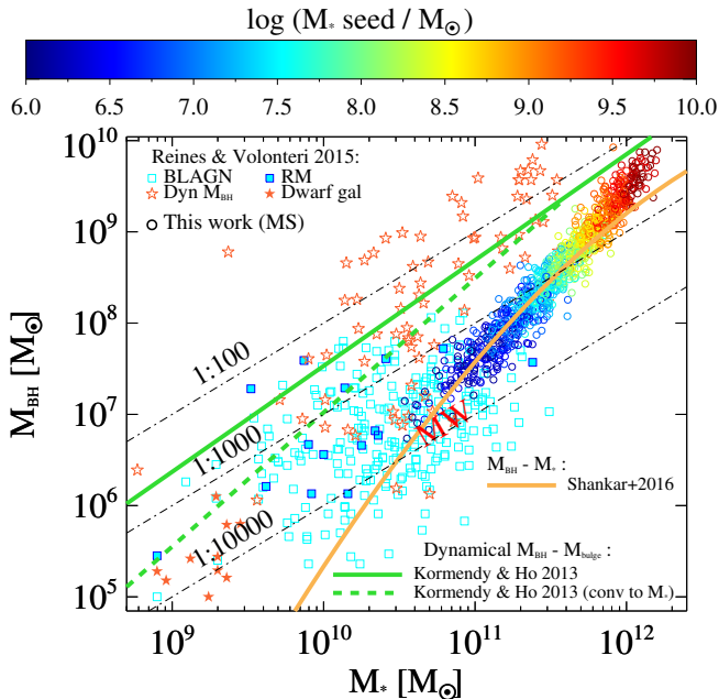
Figure 3. Final M_{\text{BH}}-M_{\star} relation at z=0 determined by our M_{\star} -dependent BHAR/SFR. The colorbar indicates the seed M_{\star} distribution at z_f . For comparison, we show the local relation from Kormendy & Ho (2013), both with M_{\text{bulge}} (green solid line) and converted to total M_{\star} (green dashed line). Our MS wedge agrees remarkably well with the proposed de-biased M_{\text{BH}}-M_{\star} trend (Shankar et al. 2016, yellow solid line) and with the virial M_{\text{BH}} estimates for BLAGN (empty squares, Reines & Volonteri 2015). For completeness, we report M_{\text{BH}}-M_{\star} estimates collected from Reines & Volonteri (2015) for reverberation mapping AGN (RM, filled squares), dynamical M_{\text{BH}} measurements (empty stars) and dwarf galaxies (filled stars). The tag “MW” marks the mass measurements for the Milky Way.
