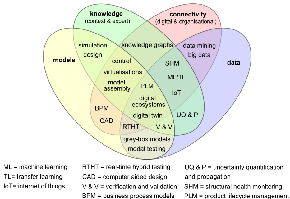
Figure 1. Diagram of the interactions between subject disciplines and technologies that form a digital twin.
