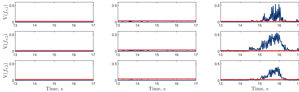
Figure 8. Digital twin \mathcal{M}^{GP}(\{\mathcal{M}^l(F, \theta_{\mathcal{D}_1}^{MAP}), F\}, \hat{\phi}_{\mathcal{D}_1}) predictive variance (—), trained using dataset one \mathcal{D}_1 , between 13 and 17s on datasets one to three (left to right); threshold (—) determined by the maximum variance from the first 100 data points on dataset two.
