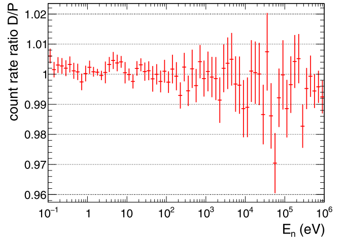
Fig. 12. Ratio of the fission count rates for dedicated (D) and parasitic (P) beam pulse types.
