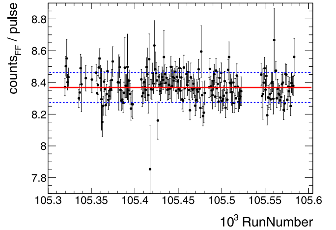
Fig. 11. Variation of the gain over time: number of events with \text{amp} > 0.1\text{ V} and E_n < 0.8\text{ MeV} per protons per run — typically 4 h per run. The red line corresponds to the weighted average of 8.36 FF counts per pulse with an uncertainty of the fit of 0.1%. The blue dashed lines indicate the standard deviation of the data points which is 1%.
