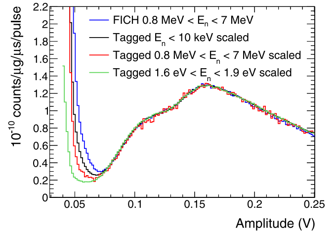
Fig. 17. Pulse height spectra of the events in the fission chamber for 0.8\text{ MeV} < E_n < 7\text{ MeV} compared to tagged events for different E_n regions from all FICH channels. The neutron flux of n_{TOF} can be seen in Fig. 7.
