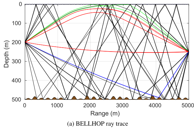
FIGURE 8. Example of a sinusoidal bathymetry with 200m long hills and random hill height between 0 and 20 m.
