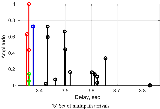
FIGURE 9. Rough sea surface and uneven seabed result in a significant increase in the number of ray-traced multipath components at the receiver, compared with the flat seabed used to obtain the results in Figure 3 and 7.
