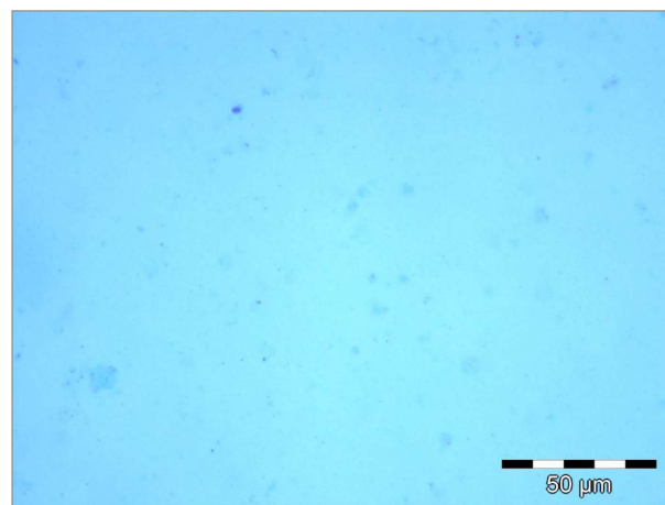
Figure 20. Microscopy image of TEPs in TSP aerosol particles sampled at the CVAO between 29 and 30 September with a flow rate of 8 L min -1 .
