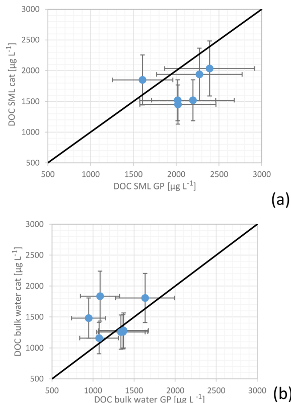
Figure 15. (a) Concentrations of DOC in the SML and (b) and in the bulk water sampled for paired glass plate (GP) and the MarParCat (cat) sampling events.
