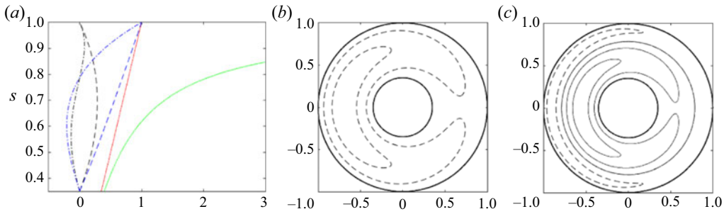
FIGURE 1. Spherical case for the Malkus field \bar{B} = s and \bar{U} = 0 . (a) Profiles of \bar{B} (red solid curve), \beta (green solid), \Phi for n = 1 (black dashed) and n = 2 (black dashed-dotted), and \Phi^\dagger for n = 1 (blue dashed) and n = 2 (blue dashed-dotted). (b,c) Streamfunctions \psi of the single-soliton solution for (b) n = 1 and (c) n = 2 , provided \epsilon = 0.1 . The dashed (solid) contour lines represent its negative (positive) value, i.e. clockwise (anticlockwise).
