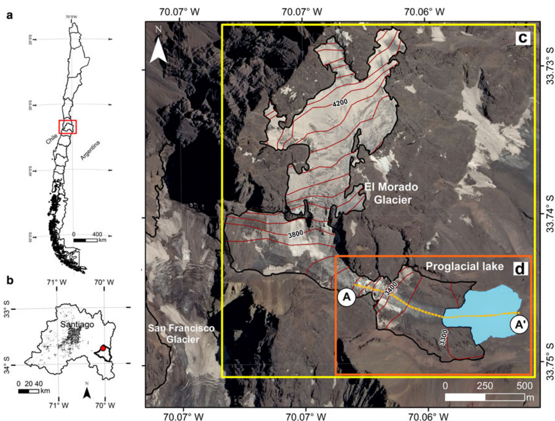
Fig. 1. Location (a) and spatial extent (b) of the Maipo River basin, central Chile. The Volcan sub-basin is highlighted within (b) along with the location of El Morado Glacier (red dot). The spatial extent of the glacier elevation and mass changes presented for the entire glacier and the glacier tongue is indicated in (c) and (d), respectively. The longitudinal profile A-A', which covers the glacier tongue and its adjacent proglacial lake, is shown in Figure 9.
