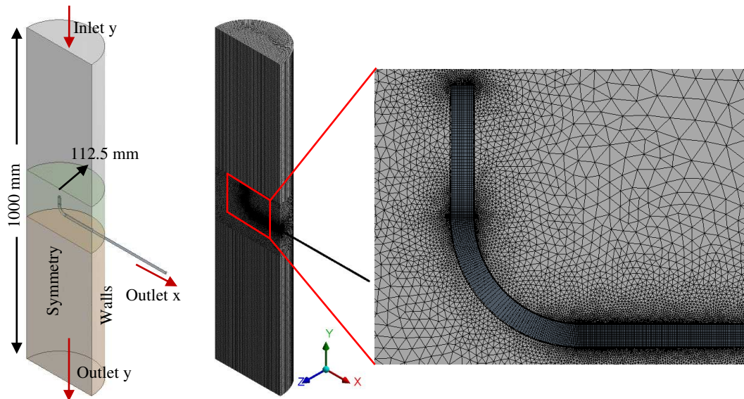
FIGURE 3: 3D schematic of the probe flow simulation and its domain with computational grid.
