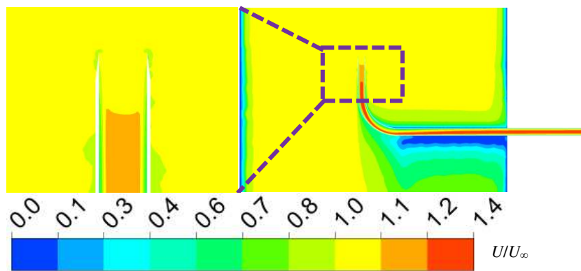
FIGURE 7. Velocity magnitude contours at the nozzle inlet.
