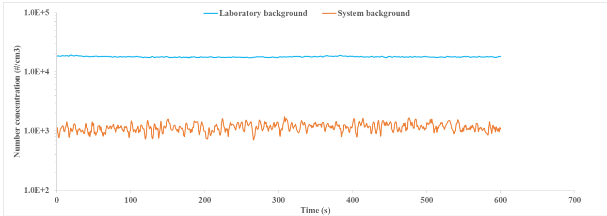
FIGURE 10. Comparison of particle concentrations in the laboratory and system environments.
