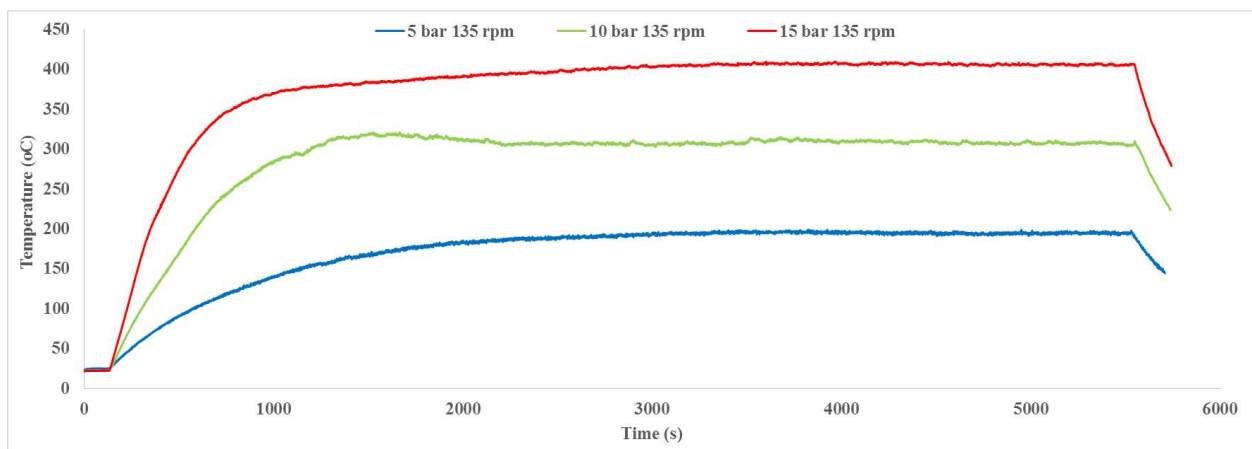
FIGURE 9. Rotor temperature variation with time for the three braking conditions.
