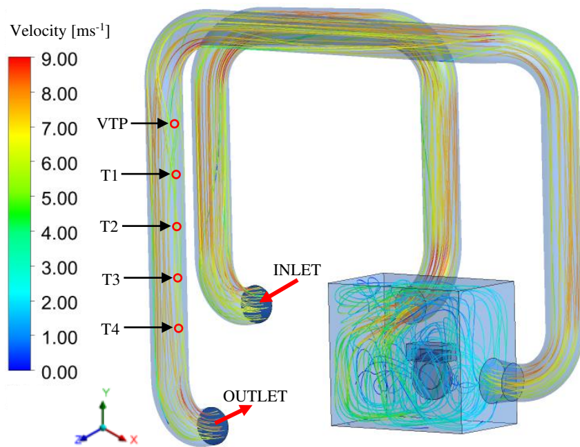
FIGURE 4. Air pathlines in the dynamometer extraction system.
