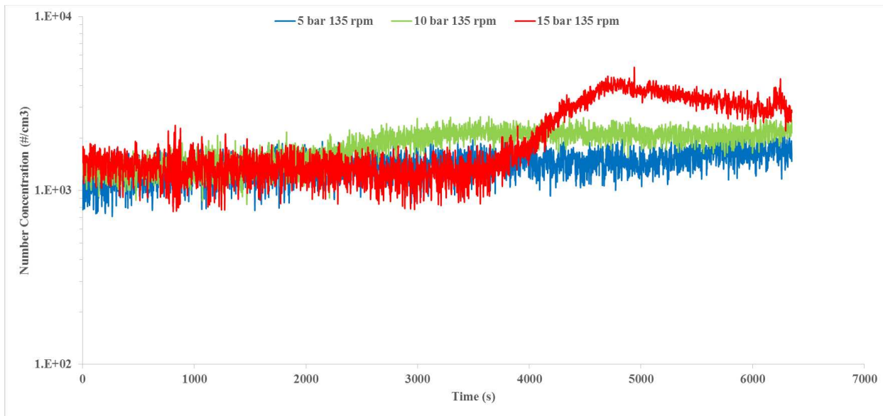
FIGURE 11. Particle concentration variation with time for the three tests.
