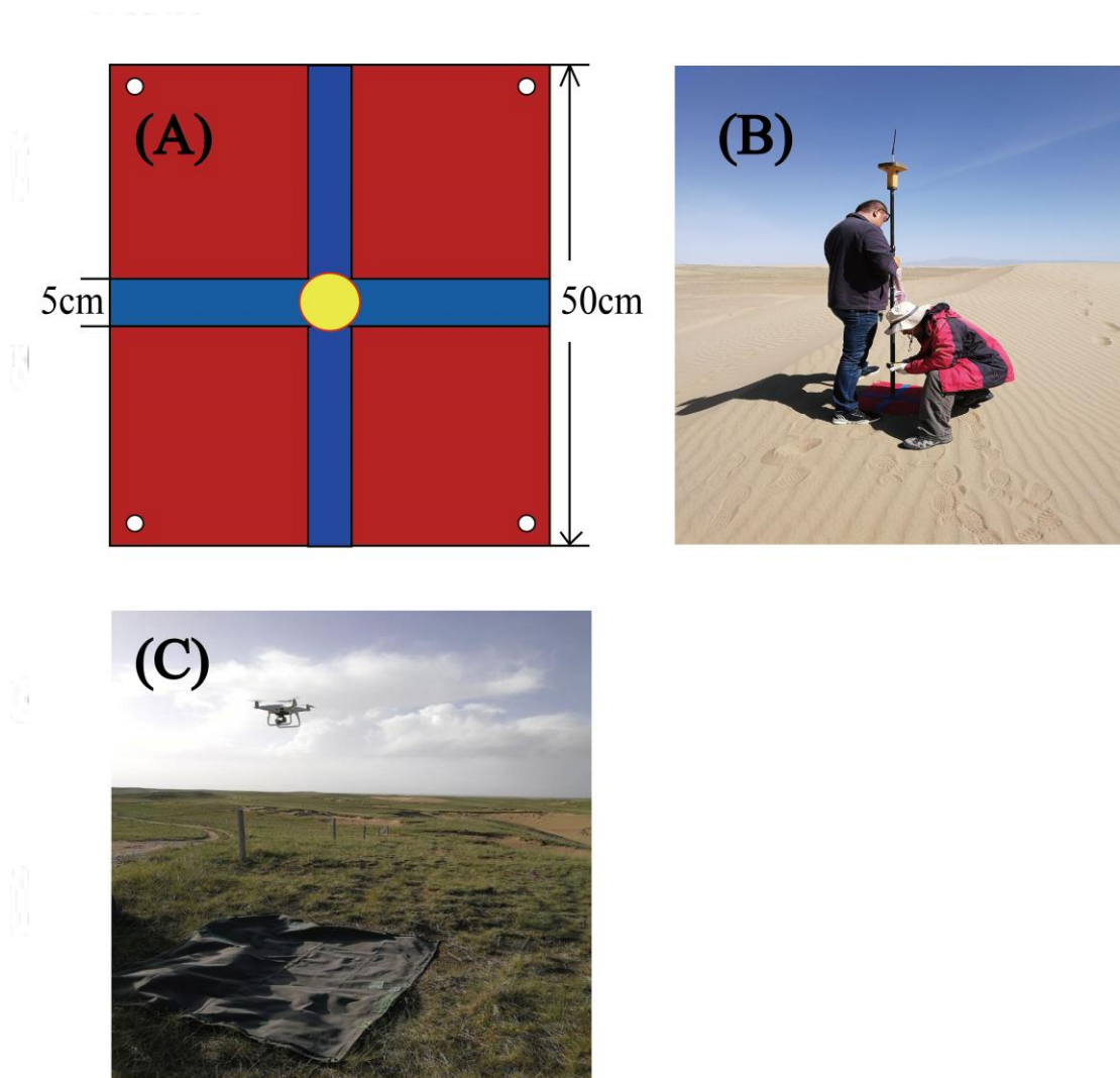
Figure 2. Pictures of the field UAV flying and measurement of the GCPs. (A) The customized GCPs sign is made of cloth material. The middle hole was used for the wooden stake to pass through, and the four corner holes were used to fix the sign. (B) The coordinate measurement of the GCPs. (C) Picture of the UAV performing a flight mission.
