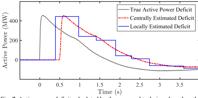
Fig. 7. Active power deficit calculated by the proposed technique based on the frequency measurement at Bus 10.
