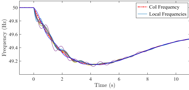
Fig. 3. Local frequencies following the outage of Generator 5.
