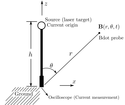
Figure 1. Schematic of the experimental set-up. The bold line represents the target holder (see Fig. 2 for the various holder designs used). During a laser shot, charge accumulation in the target generates a return current that propagates down the target holder. The magnetic field is measured by a B-dot probe and the neutralization current is recorded using an oscilloscope connected by a coaxial cable to the base of the holder.
