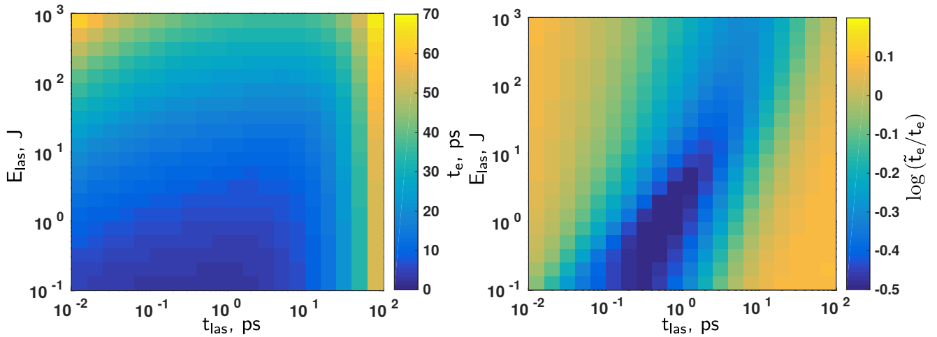
Figure 9. (Color online) Comparison of two methods of computing the charging time, t_e , for copper targets. The laser FWHM is 10\ \mu\text{m} , with laser absorption \eta = 40\% . The target is assumed infinite. Left plot: Values of t_e computed using ChoCoLaTII.f90. The charging time is defined as the moment when the target has accumulated 80% of its total charge. Right plot: Logarithm of the ratio between Eq. (3) and ChoCoLaTII.f90 values from the left plot.
