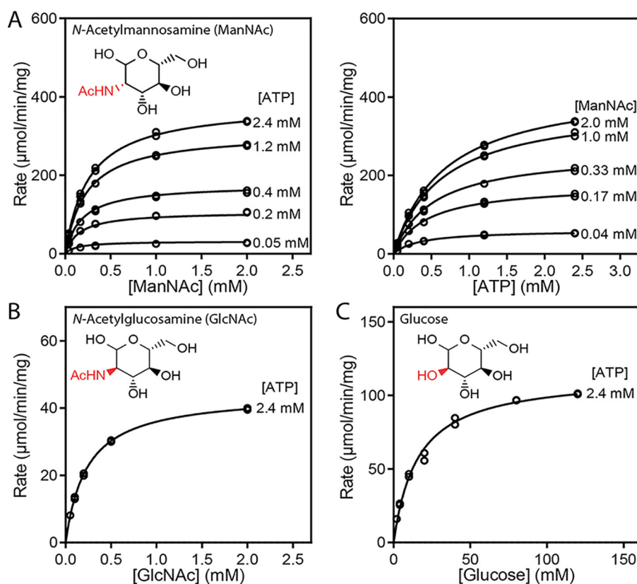
Figure 2. Kinetic assays with N-acetylmannosamine kinase. A, rate versus N-acetylmannosamine and ATP concentration fitted with the ternary complex kinetic model: K_m (N-acetylmannosamine) = 0.30 \pm 0.01 mM, K_m^{\text{ATP}} = 0.7 mM, V_{\text{max}} = 497 \pm 7 \mu\text{mol}/\text{min}/\text{mg} , k_{\text{cat}} = 263 \pm 3 \text{s}^{-1} . B, rate versus GlcNAc concentration fitted to the Michaelis-Menten model: K_m^{\text{PP}} = 0.26 mM, V_{\text{max}} = 114 \mu\text{mol}/\text{min}/\text{mg} , k_{\text{cat}}^{\text{PP}} = 23.4 \pm 0.2 \text{s}^{-1} . C, rate versus glucose concentration fitted to the Michaelis-Menten model: K_m = 15 \pm 1 mM, V_{\text{max}} = 44.4 \pm 0.3 \mu\text{mol}/\text{min}/\text{mg} , k_{\text{cat}} = 60 \pm 1 \text{s}^{-1} .
