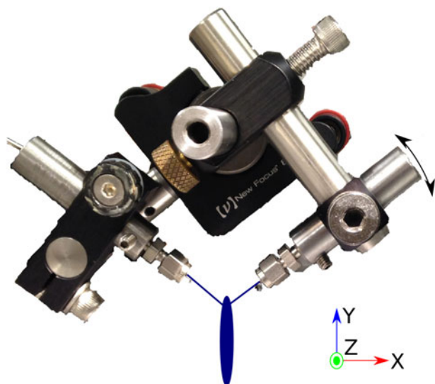
Fig. 1. The experimental setup to create the liquid films, showing the axes we use when talking about the liquid window. The skew of the window was controlled by offsetting the nozzles in Z, and the effect of changing the other axes is negligible in comparison.
