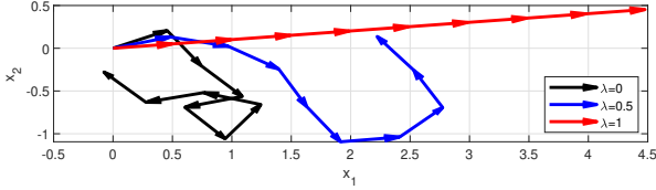
Fig. 2. The movement of the peak center through a 2-dimensional subspace over 10 environmental changes where \tilde{s} = 1 . The initial position of peak is [0,0] , and the same random seed is used for each sequence of movements.
