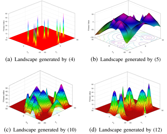
Fig. 1. Landscapes with 10 components generated by different baselines. All shared parameter settings, such as component centers' locations, heights, and widths, are equal. In Figure 1(c), \beta is set to zero. Note that in contrary to the flat regions in Figure 1(c) whose gradient is zero, the gradients in the flat looking regions in Figures 1(a) and 1(d) have positive non-zero values.
