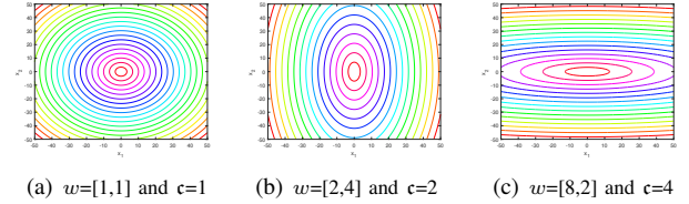
Fig. 8. Three different 2-dimensional components with different ill-conditioning degrees. The values of widths ( w ) of each peak and their corresponding condition number ( c ) are shown.
