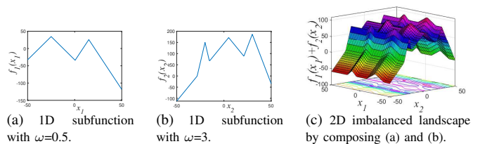
Fig. 14. Imbalanced landscape generated by composing two subfunctions with different weights \omega in (32).
