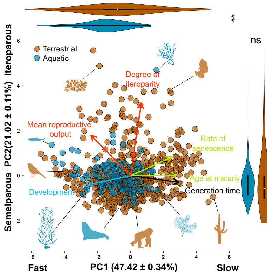
FIGURE 2 Aquatic and terrestrial life-history strategies are organized in two main axes of variation, the fast–slow continuum and the reproductive strategies. Trait definitions are in Table 1. Phylogenetically corrected principal component analysis (pPCA) for the first two axes (percentage of variance absorbed in brackets \pm SE) for six key life-history traits from 122 aquatic (blue) and 685 terrestrial species (brown). Arrow lengths indicate mean loading of each life-history trait, and colour indicates associations with population turnover (black), survival (green), development (blue) and reproduction (red). Each point represents the mean position of a species on this two-dimensional space for 10 imputed datasets (see Methods). Violin plots (top and right) depict the distribution of species along each principal component axis; white dot: mean; black thick line: 25th–75th quantile; black thin line: SD; ns, not-significant; * p < 0.01 ; ** p < 0.005 . The silhouettes, starting at the top left and moving anticlockwise, correspond to: Lantana camara , Clinostomus funduloides , Setophaga cerulea , Pterygophora californica , Mirounga leonina , Gorilla beringei , Paramuricea clavata , Pseudomitrocereus fulviceps , Cyripedium calceolus and Gracilaria gracilis
