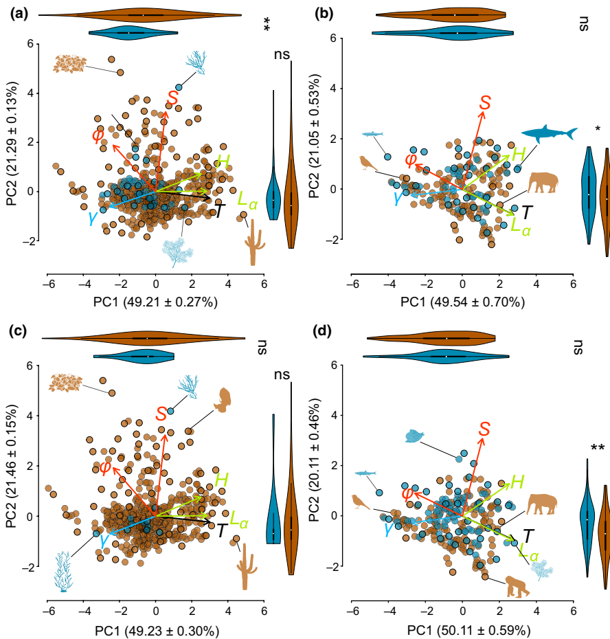
FIGURE 3 The main axes of life-history variation remain constant, regardless of the degree of mobility/sessility or taxonomic kingdom. Phylogenetically corrected principal component analysis of six life-history traits across 683 species are shown in Table 1. Note that the fast-slow continuum remains the dominant axis of variation across all partitions, explaining 49%–50% of the variation, followed by an axis of reproductive strategies, which explains ~21% of the variation in life-history traits. ns, non-significant; * p < 0.05 ; ** p < 0.01 . (a) Sessile organisms, with silhouettes (starting at the top left and moving anticlockwise) representing: Lantana camara , Paramuricea clavata , Pseudomitrocereus fulviceps and Gracilaria gracilis . (b) Mobile organisms: Clinostomus funduloides , Setophaga cerulea , Elephas maximus and Isurus oxyrinchus . (c) Kingdom Plantae and Chromista: L. camara , Pterygophora californica , P. fulviceps , C. calceolus and G. gracilis . (d) Kingdom Animalia: Mya arenaria , C. funduloides , S. cerulea , Gorilla beringei , P. clavata and E. maximus
