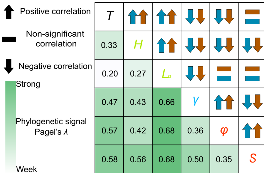
FIGURE 1 Trade-offs among life-history traits are congruent between aquatic and terrestrial environments. Pairwise correlations between six life-history traits (Table 1) for 122 aquatic (blue) and 685 terrestrial (brown) species. Arrows indicate the direction of each pairwise correlation using phylogenetic generalized least squares: positive (arrow-up), negative (arrow-down) or not-significant correlation (horizontal bar; p > 0.05 ). The mean phylogenetic signal (Pagel's \lambda ) of each pairwise correlation, displayed in the lower triangle, ranges from weak (white, ~0.00) to strong (dark green, ~1.00)
