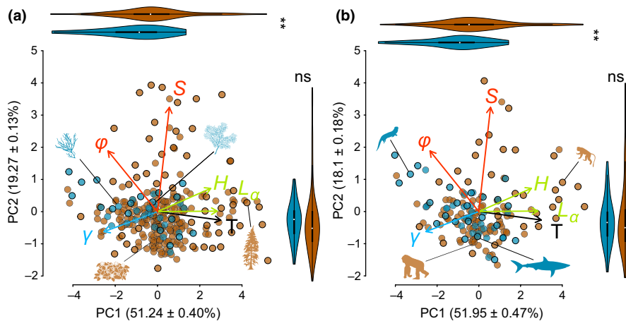
FIGURE 4 The main axes of life-history variation remain constant in sessile (a) and mobile (b) species when correcting by maximum body size (m) and adult body mass (g) respectively. Phylogenetically and size-corrected principal component analysis of six life-history traits across 464 species. Trait definitions are in Table 1. Note that the fast-slow continuum remains the dominant axis of variation, explaining ~51% of the variation, followed by an axis of reproductive strategies, which explains 18%–19% of the variation in life-history traits. ns: non-significant; * p < 0.05 ; ** p < 0.01 . (a) Sessile organisms, with silhouettes (starting at the top left and moving anticlockwise) representing: Gracilaria gracilis , Lantana camara , Pinus ponderosa and Paramuricea clavata . (b) Mobile organisms: Enhydra lutris , Gorilla beringei , Isurus oxyrinchus and Presbytis thomasi
