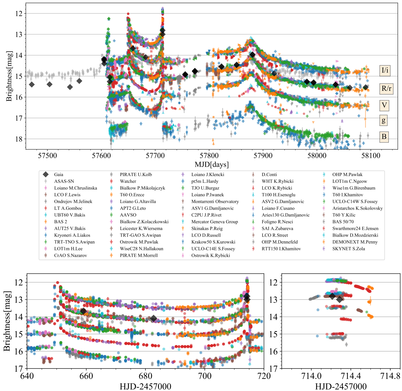
Fig. 2. Gaia, ASAS-SN, and follow-up photometric observations of Gaia16aye. Each observatory and observer is marked with a different colour. The marker is explained in the legend. The figure shows only the follow-up data, which were automatically calibrated using the Cambridge Photometric Calibration Server. The upper panel shows the entire event, and the bottom panels show a zoom on the second pair of caustic crossings (left) and a detail of the fourth caustic crossing (right).
