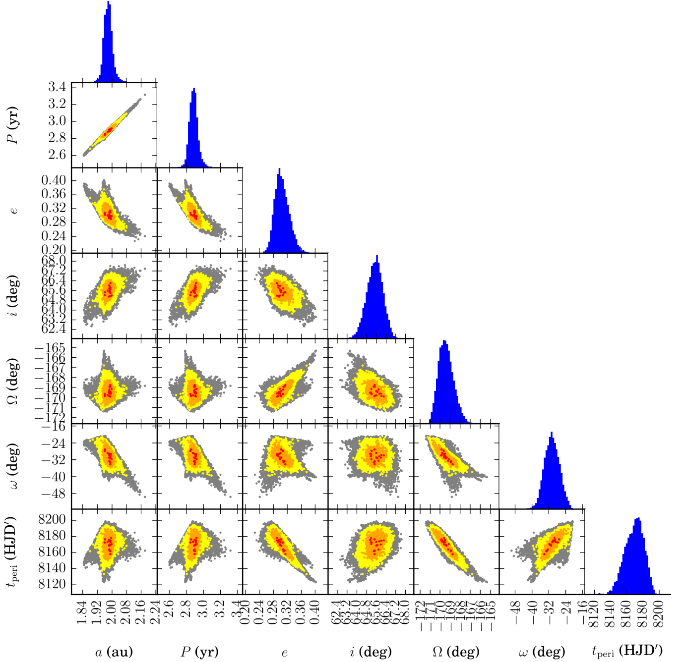
Fig. 9. Orbital elements of Gaia16aye. The panels show 2D and 1D projections of posterior distributions in the space of Kepler parameters. Red, orange, and yellow points mark 1\sigma , 2\sigma , and 3\sigma confidence regions, respectively.
