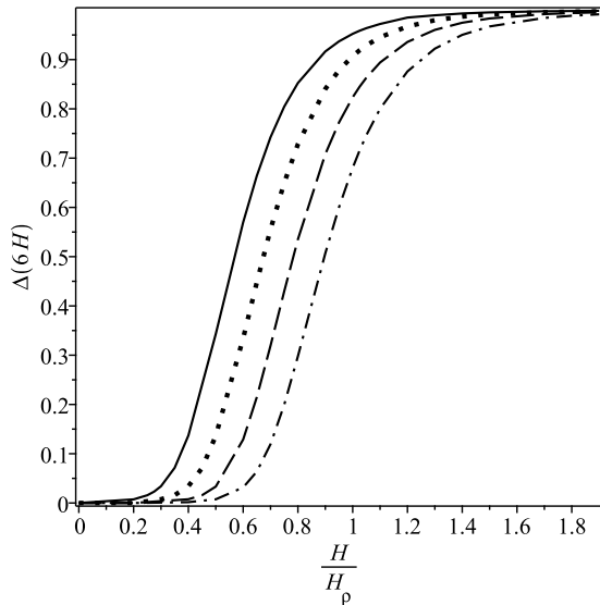
Fig. 4. Dependence of \Delta(6H) on the ratio H/H_\rho for \zeta = 5 , r_0/H = 0.1 , and \nu = 10^7 \text{ m}^2 \text{ s}^{-1} . The solid line corresponds to H = 30 \text{ Mm} and the wave period 60 s. The dotted line corresponds to H = 60 \text{ Mm} and the wave period 60 s. The dashed line corresponds to H = 30 \text{ Mm} and the wave period 30 s. The dash-dotted line corresponds to H = 60 \text{ Mm} and the wave period 30 s.
