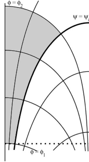
Fig. 1. Sketch of domain \mathcal{D} . The coordinate lines are shown in the plane \theta = \text{constant} . The vertical curves are the magnetic field lines defined by the equation \psi = \text{constant} . The horizontal curves are defined by the equation \phi = \text{constant} . The thick vertical curve is the boundary of the region where the wave propagation is considered. It is defined by the equation \psi = \psi_b ; \phi_1 = -H and \phi_2 = -He^{-6} . It is assumed that the waves are driven at the line \phi = \phi_1 . The dotted line shows the level z = 0 .
