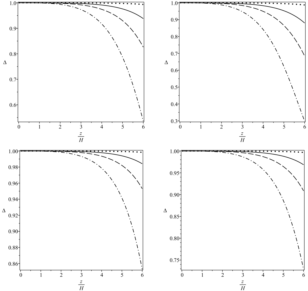
Fig. 3. Dependence of the relative wave energy flux \Delta on the height z . Upper panels: wave period 30 s, lower panels: wave period 60 s. Left panels: H = 30 Mm, right panels: H = 60 Mm. The dotted, solid, dashed, and dash-dotted lines correspond to \nu = 10^5 \text{ m}^2 \text{ s}^{-1} , 10^6 \text{ m}^2 \text{ s}^{-1} , 3 \times 10^6 \text{ m}^2 \text{ s}^{-1} , and 10^7 \text{ m}^2 \text{ s}^{-1} .
