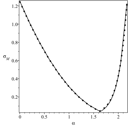
Fig. 2. Dependence of \sigma_M on \alpha for \zeta = 5 . The solid line shows the numerically calculated dependence, and the squares show the graph of the approximate dependence \sigma_M on \alpha given by Eq. (48).
