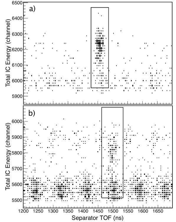
Fig. 1. Plot of total IC energy vs. separator TOF for data passing additional software cuts (see text) for a) E_{cm} = 5.713 MeV and b) E_{cm} = 5.415 MeV data. The IC energy and separator TOF cuts showing the regions of interest are also indicated.
