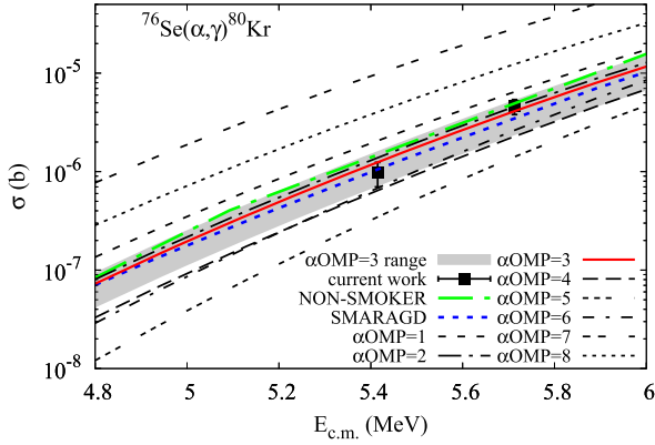
Fig. 2. Cross section data ( \sigma ) obtained in this work compared with those calculated with TALYS, SMARAGD, and NON-SMOKER. The gray-shaded area denotes range of uncertainty in the cross section from \alpha OMP=3 obtained by scaling up and down the red curve to overlap with the 68% confidence level of the experimental data.
