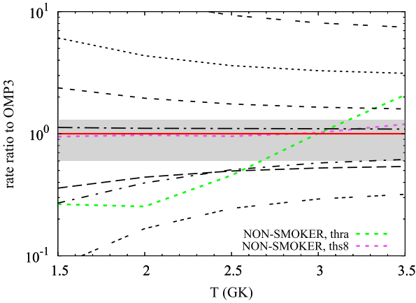
Fig. 3. Ratio of reaction rates from Talys to that obtained with \alpha OMP=3. Line styles and colors correspond to those used in Fig. 2. The green and magenta dashed lines indicate rates from REACLIB database that correspond to two different parametrizations of the NON-SMOKER results. See text for details. The gray shaded area correspond to the uncertainty in the \alpha OMP=3 cross section. SMARAGD reaction rate data was not available.
