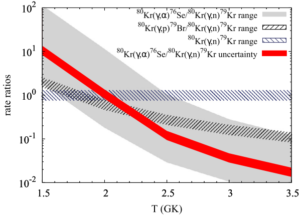
Fig. 4. Ratios of (\gamma, \alpha) and (\gamma, p) rates to (\gamma, n) rates obtained with Talys. Gray shaded band is the uncertainty in the (\gamma, \alpha)/(\gamma, n) ratio obtained from Talys. The red band corresponds to the (\gamma, \alpha)/(\gamma, n) ratio resulting from this work. The dashed regions indicate the (\gamma, p)/(\gamma, n) ratio (black) and the uncertainty in the (\gamma, n) rate (blue).
