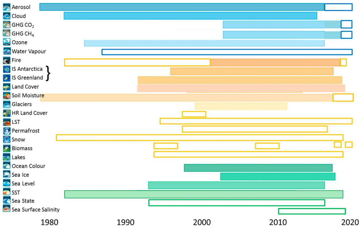
Fig. 1. Temporal coverage of CDRs for ECVs analyzed by CCI. Filled bars indicate CDRs available in 2019, and outlined bars indicate CDRs that are planned within the ongoing phase of the CCI program.
