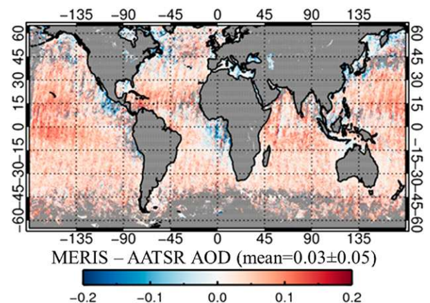
Fig. 5. Mean AOD differences at 865 nm between ocean-color MERIS atmospheric correction by-product and aerosol ECV product from AATSR in May 2003 when both instruments retrieve AOD.
