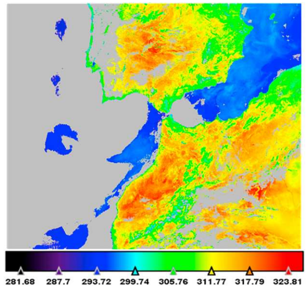
Fig. 3. Gaps in surface temperature fields (LST and SST from SLSTR on Sentinel-3A at 1038 UTC 5 Aug 2018) due to masked clouds (gray), showing the absence of scatter at land–sea borders and sampling discontinuities across some land–sea boundaries due to different cloud-clearing approaches between LST and SST processing.
