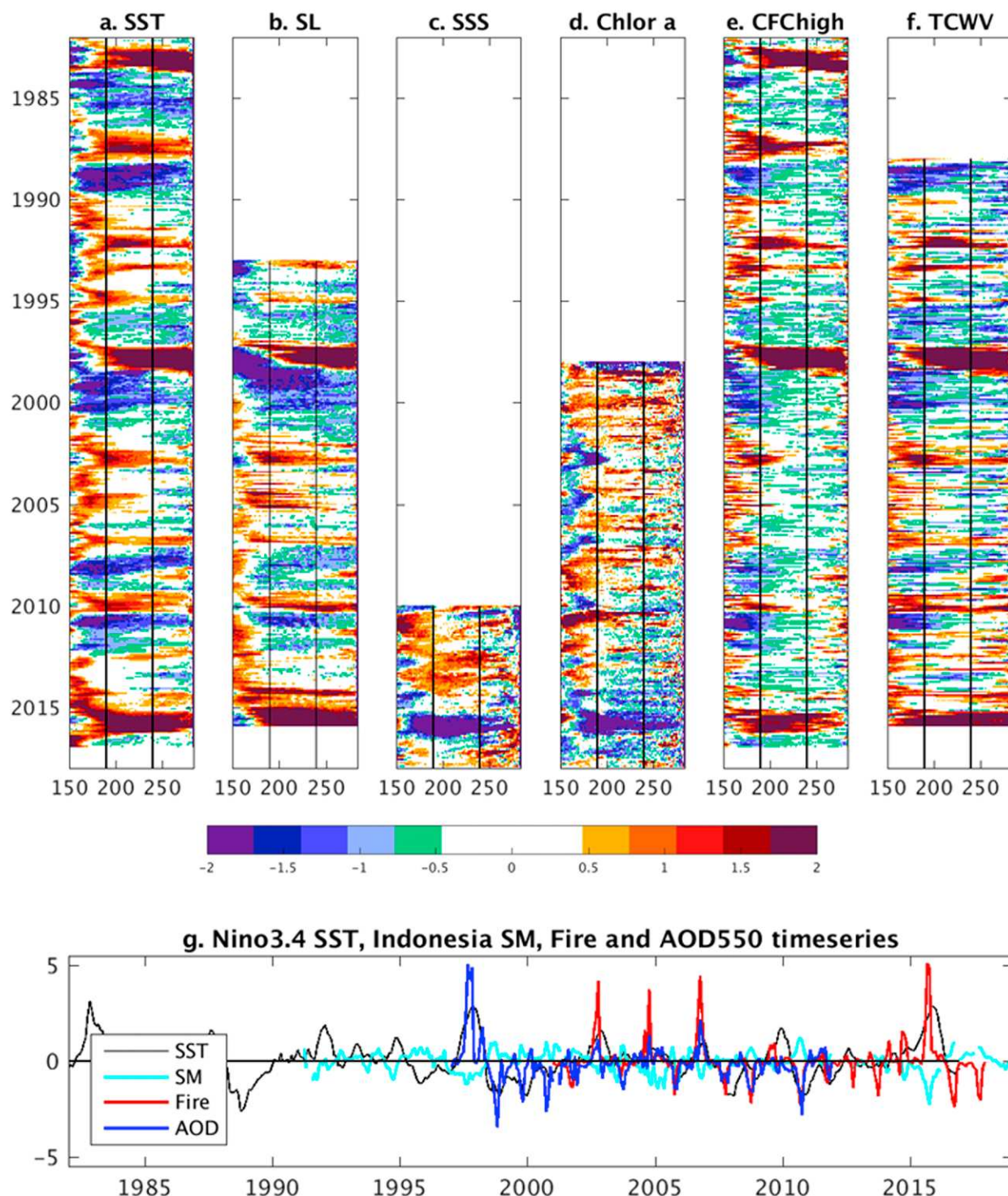
Fig. 10. Zonal month-longitude cross sections (averaged between 5°S and 5°N) for 150°E–280°E normalized indices of (a) sea surface temperature (SST), (b) sea level height (SL), (c) sea surface salinity (SSS), (d) chlorophyll-a (Chlor_a), (e) high-level cloud fraction (CFChigh), and (f) total-column water vapor (TCWV). All ECVs are plotted for their respective full-year availability. The black lines in the Hovmöller plots show the Niño-3.4 box. (g) Time series of Niño-3.4 SST and Indonesia soil moisture (SM), burned area (Fire), and aerosol optical depth at 550 nm (AOD550). Information on the used datasets is provided in Table A1 in the appendix.
