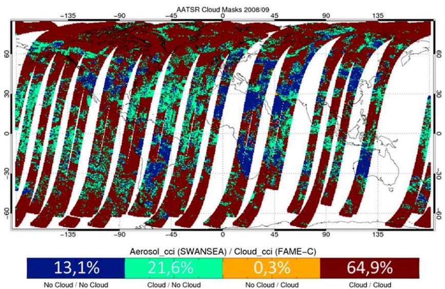
Fig. 4. Consistency overview between Aerosol_cci (Swansea University) and Cloud_cci (FAME-C) AATSR cloud masks for observations of four selected days in September 2008. “No cloud/no cloud” and “cloud/cloud” situations are solely analyzed as aerosol or clouds in Aerosol_cci and Cloud_cci, respectively. “No cloud/cloud” situations are wrongly analyzed as aerosols and clouds, while “cloud/no cloud” situations are not analyzed at all.
