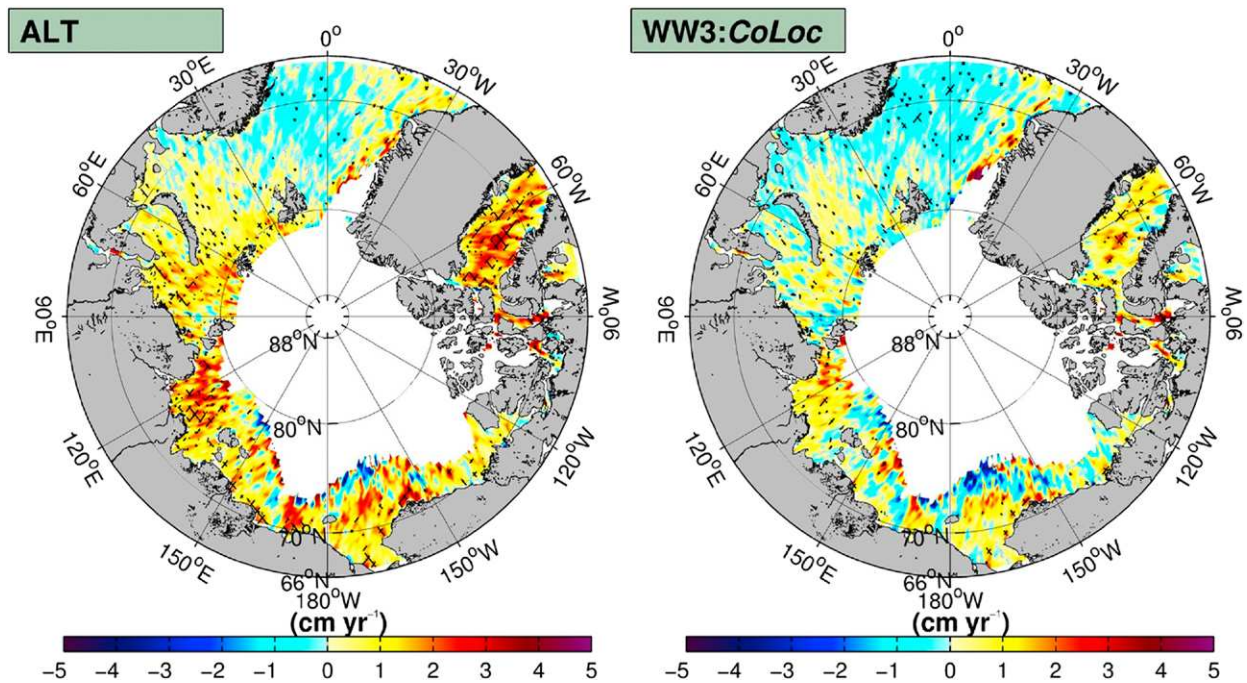
Fig. 9. Trends of monthly averaged significant wave height ( H_s ) datasets ( \text{cm yr}^{-1} ) with the Mann–Kendall test (thatched areas) from (left) satellite altimetry (ALT), and (right) collocated model WW3 hindcast (CoLoc).
