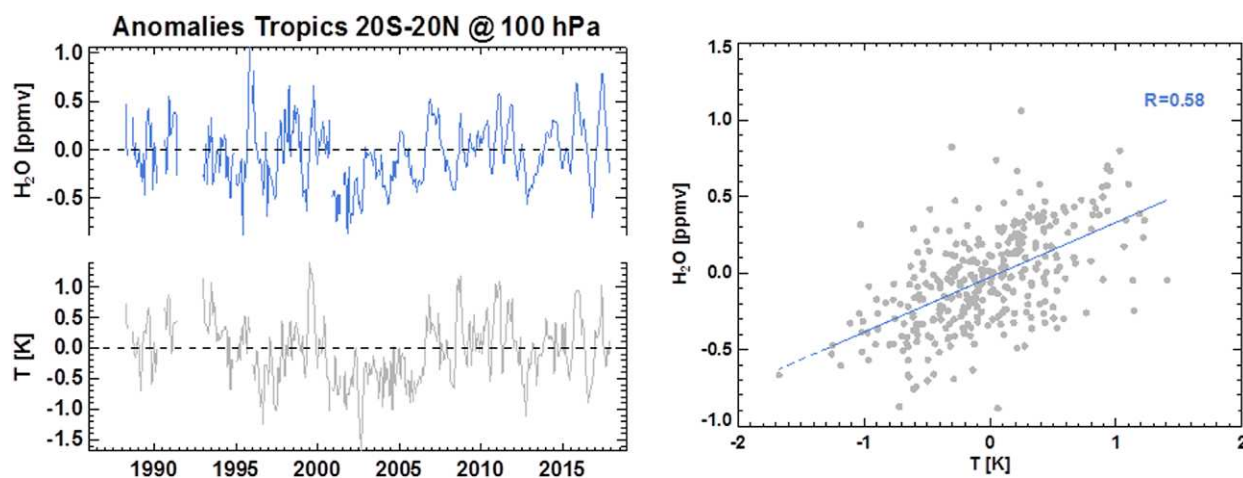
Fig. 8. (left) Covariation between a prototype version of the stratospheric water vapor CDR \text{H}_2\text{O} (produced within the Water_Vapour_cci ) and ERA5 monthly zonal mean temperatures T at 100 hPa. (right) Correlation between the two datasets.
