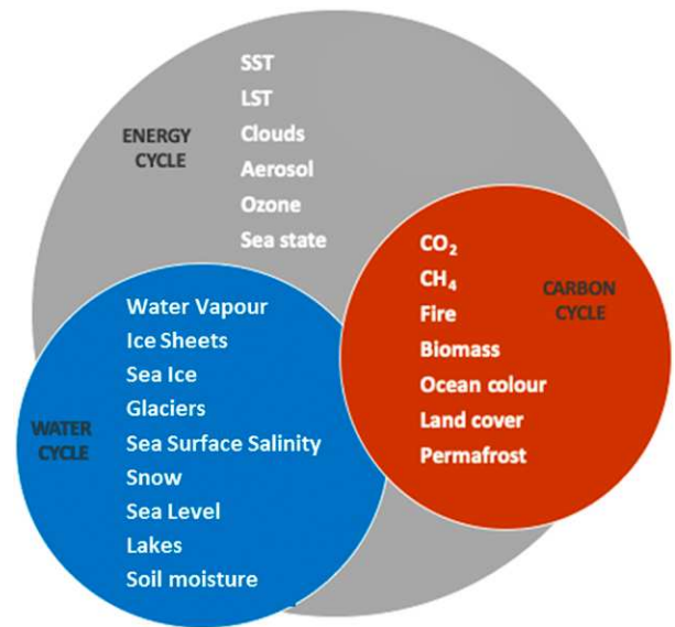
Fig. 2. The ECVs covered by ESA CCI CDRs, ordered according to the key Earth system cycle (energy, carbon, water) they help characterize. The cycles are interlinked, and most water and carbon cycle ECVs are also relevant to the energy cycle, since energy is stored and transported in water and matter, at least on transient time scales.
