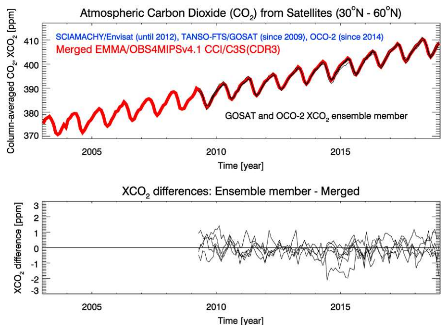
Fig. 6. (top) Time series of monthly mean northern midlatitude X_{CO_2} (red thick line) based on merging individual X_{CO_2} ensemble members (black lines) from GOSAT (since 2009) and OCO-2 (since 2014). The time series (2003–18) begins with one X_{CO_2} product from SCIAMACHY/Envisat. (bottom) X_{CO_2} difference between ensemble members (black lines) and the multisensor/multialgorithm merged product (red line in top panel). For details, see Reuter et al. (2020).
