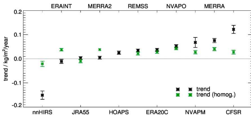
Fig. 7. Trend estimates computed after (green) and before (black) homogenization for all long-term TCWV data records available from the G-VAP data archive (Schröder et al. 2018). Trend estimates are sorted in ascending order without homogenization. The gray horizontal line marks a trend of 0 \text{kg m}^{-2} \text{yr}^{-1} (updated from Schröder et al. 2019).
