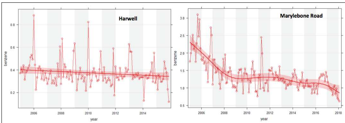
Figure 6. Deseasonalised trends in benzene ( \mu\text{g m}^{-3} ) at Harwell 2005-2015 (left) and Marylebone Road 2005-2018 (right). Data from Defra Automated Hydrocarbon network. Solid line is the trend, shaded area 95% confidence interval.
