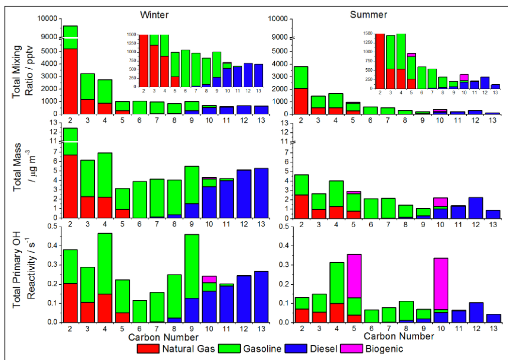
Figure 9. Contribution of different types of VOCs to mixing ratio, mass and OH reactivity in London, North Kensington, based on data from the 2012 Clearflo campaign. VOCs in the Diesel and C_{10} biogenic groups are not currently measured in the Defra hydrocarbon network, whereas Gasoline, Natural gas and Biogenic are represented by monitoring. Reproduced from Dunmore et al. Atmos. Chem. & Phys. 15 , 9983-9996, 2015.
