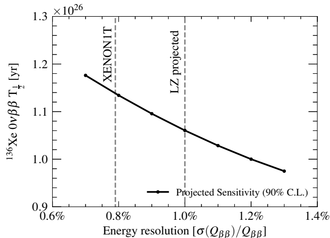
FIG. 5. Expected 90% CL sensitivity for a 1000 live-days run and for various assumed values of energy resolution at Q_{\beta\beta} . The vertical dashed line labeled “LZ projected” marks the assumed resolution for this analysis. Also shown on the plot is the projected LZ sensitivity assuming the energy resolution recently measured in XENON1T [34].
