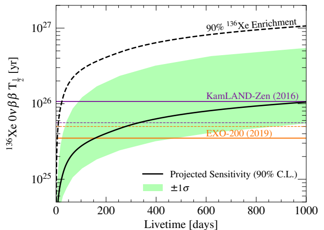
FIG. 4. LZ projected sensitivity to ^{136}\text{Xe} 0\nu\beta\beta decay as a function of detector live time. The light green shaded band represents a \pm 1\sigma statistical uncertainty on the sensitivity. The dashed black line shows the projected sensitivity to ^{136}\text{Xe} 0\nu\beta\beta decay for a dedicated run with 90% ^{136}\text{Xe} enrichment. For comparison, the limits set by EXO-200 [55] (orange full) and KamLAND-Zen [5] (purple full) are also shown, along with the respective projected sensitivities (dashed).
